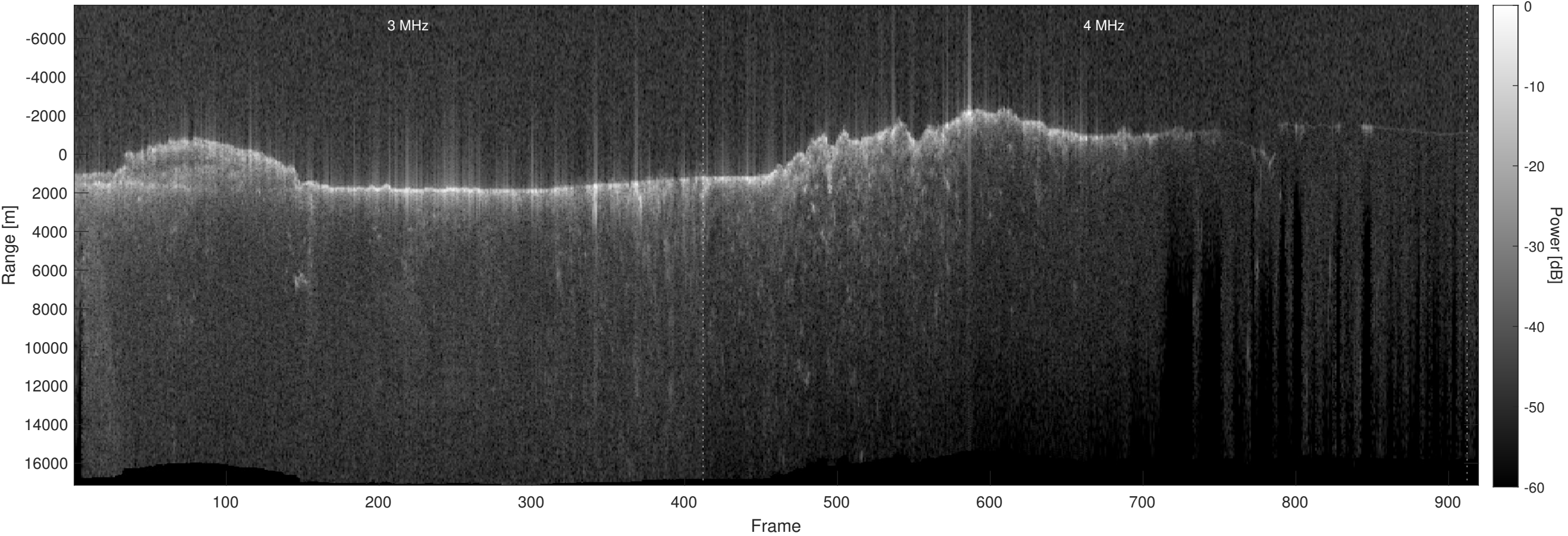
Orbit 11622, Optimized, No Window, Depth-Corrected, Channel 2
