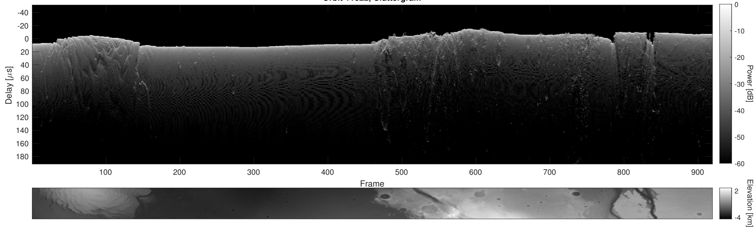
Orbit 11622, Cluttergram
