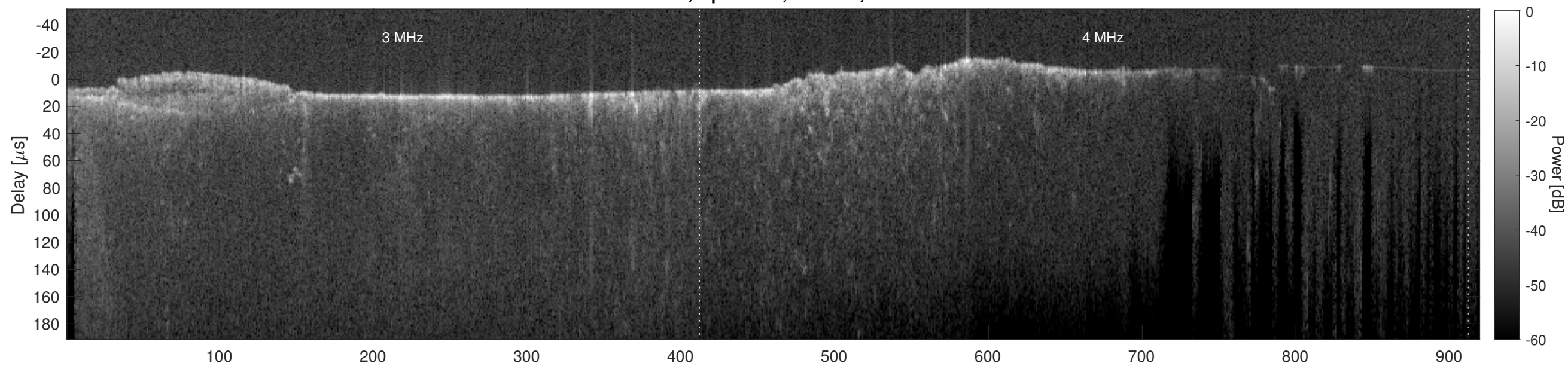
Orbit 11622, Cluttergram
