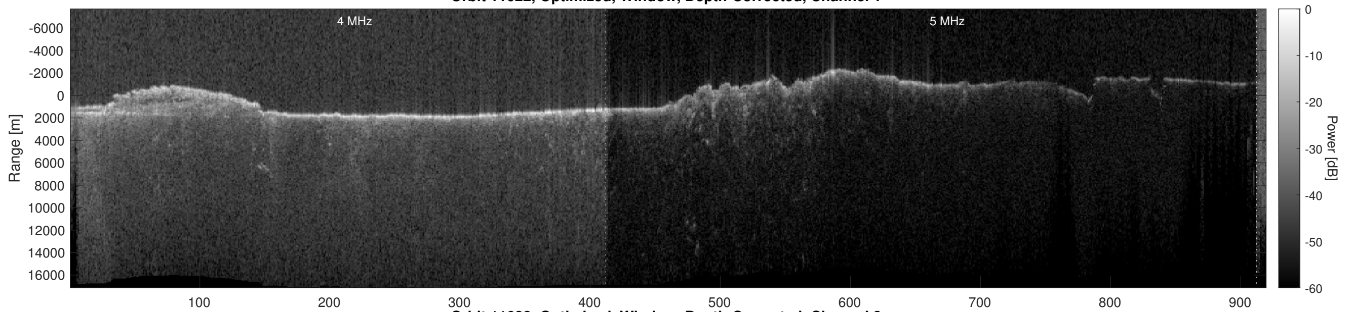
Orbit 11622, Optimized, Window, Depth-Corrected, Channel 2
