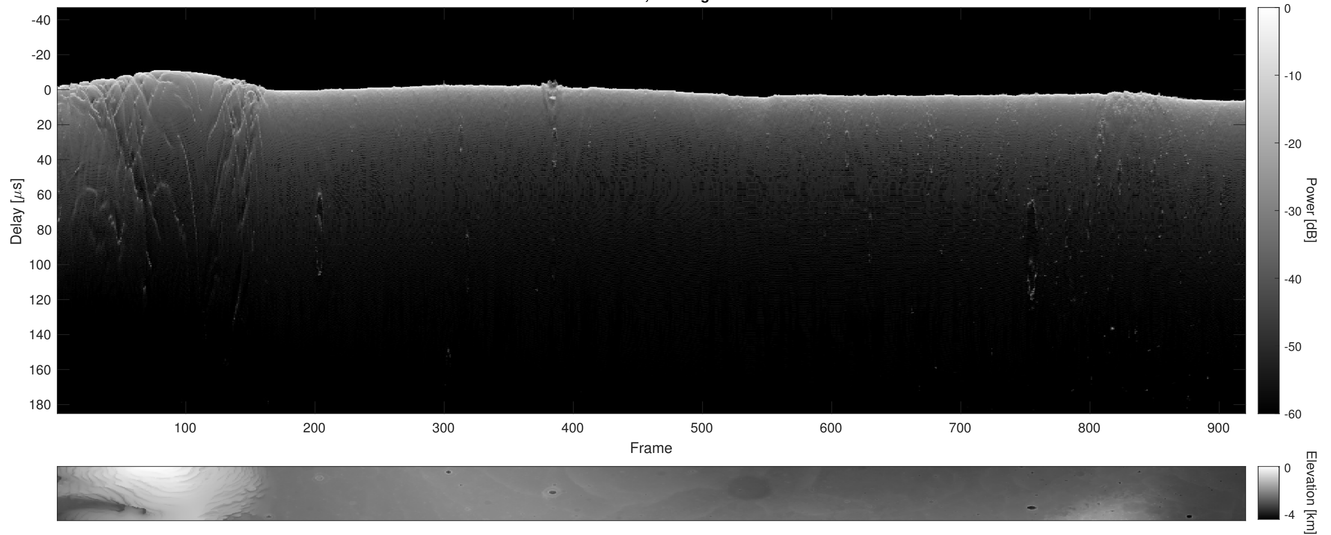
Orbit 11624, Cluttergram
