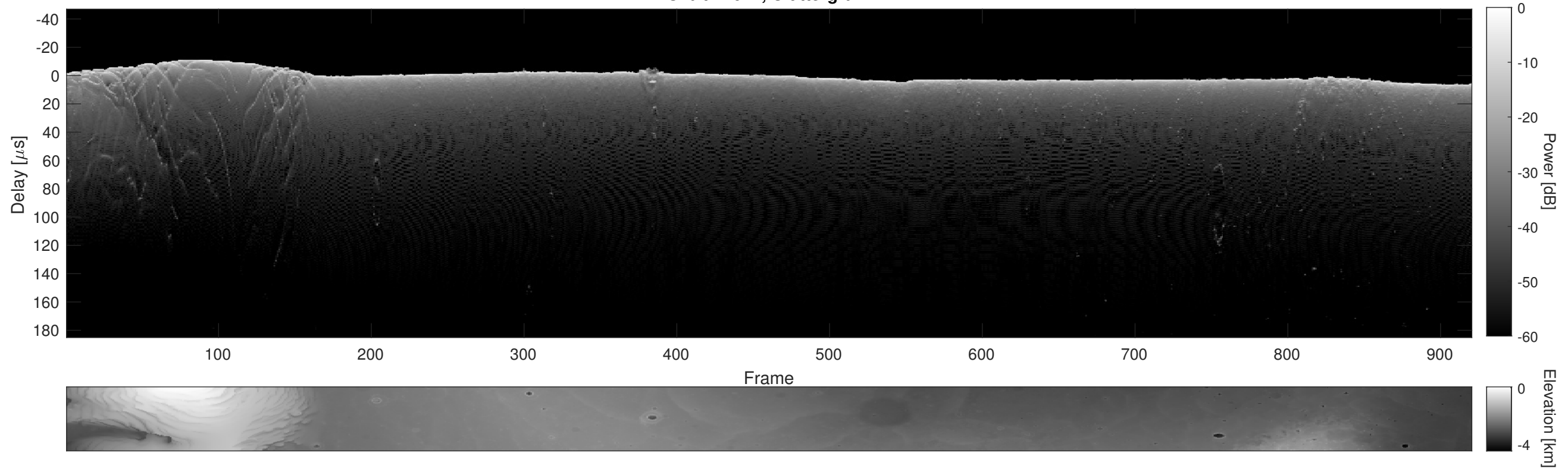
Orbit 11624, Cluttergram
