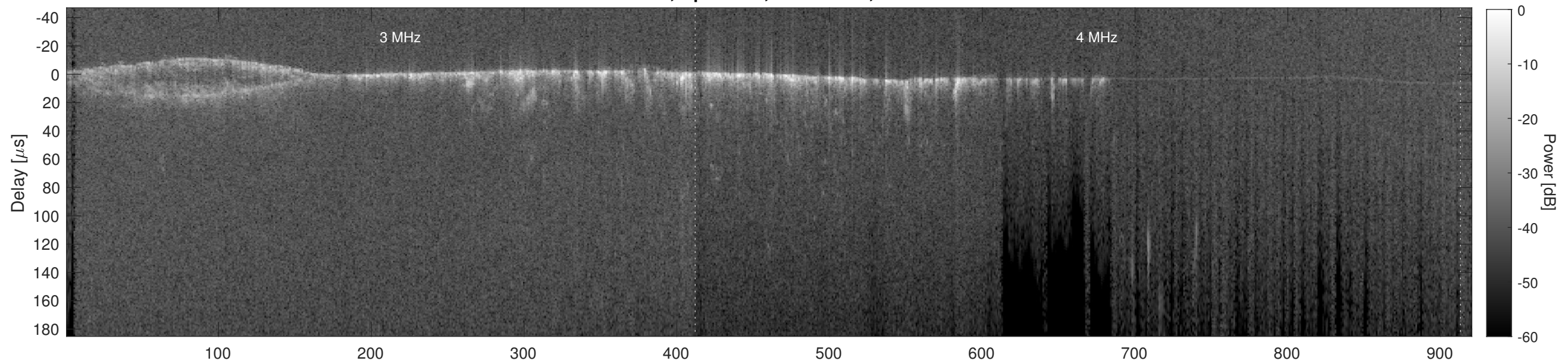
Orbit 11624, Cluttergram
