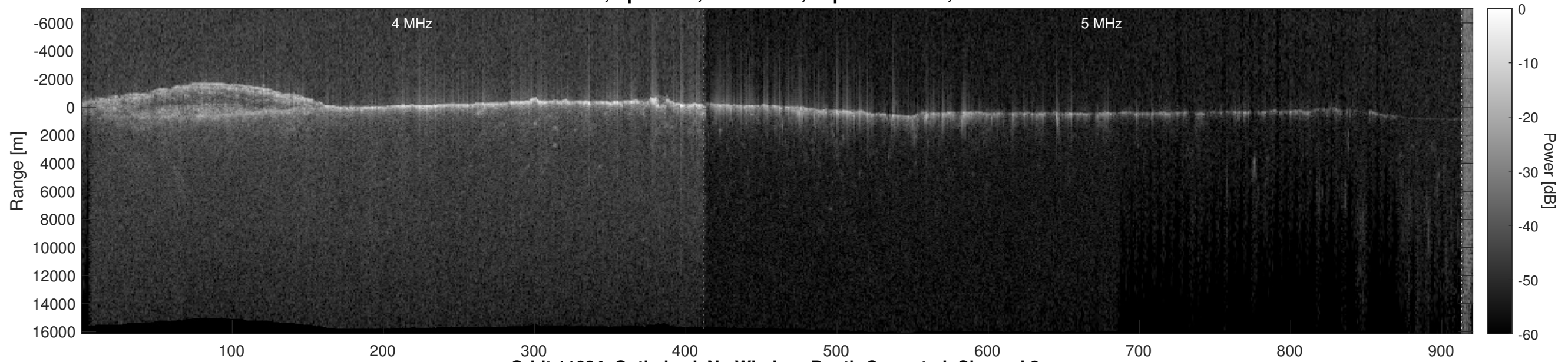
Orbit 11624, Optimized, No Window, Depth-Corrected, Channel 2
