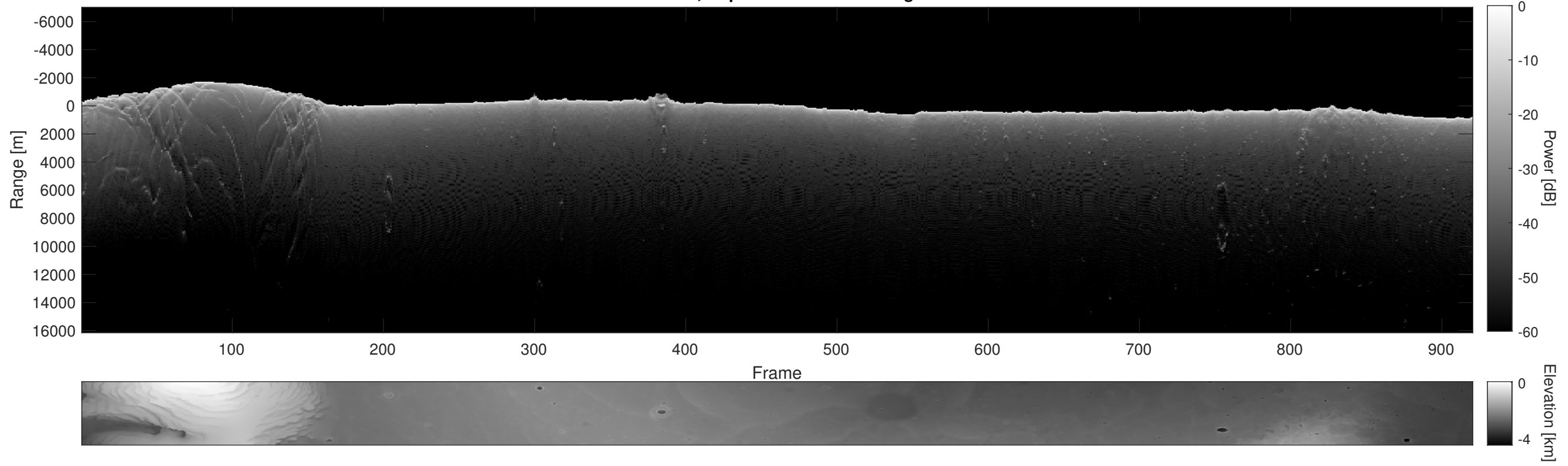
Orbit 11624, Depth-Corrected Cluttergram
