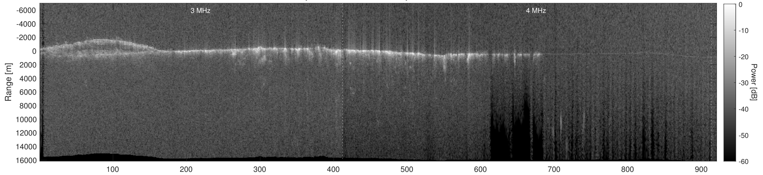
Orbit 11624, Depth-Corrected Cluttergram
