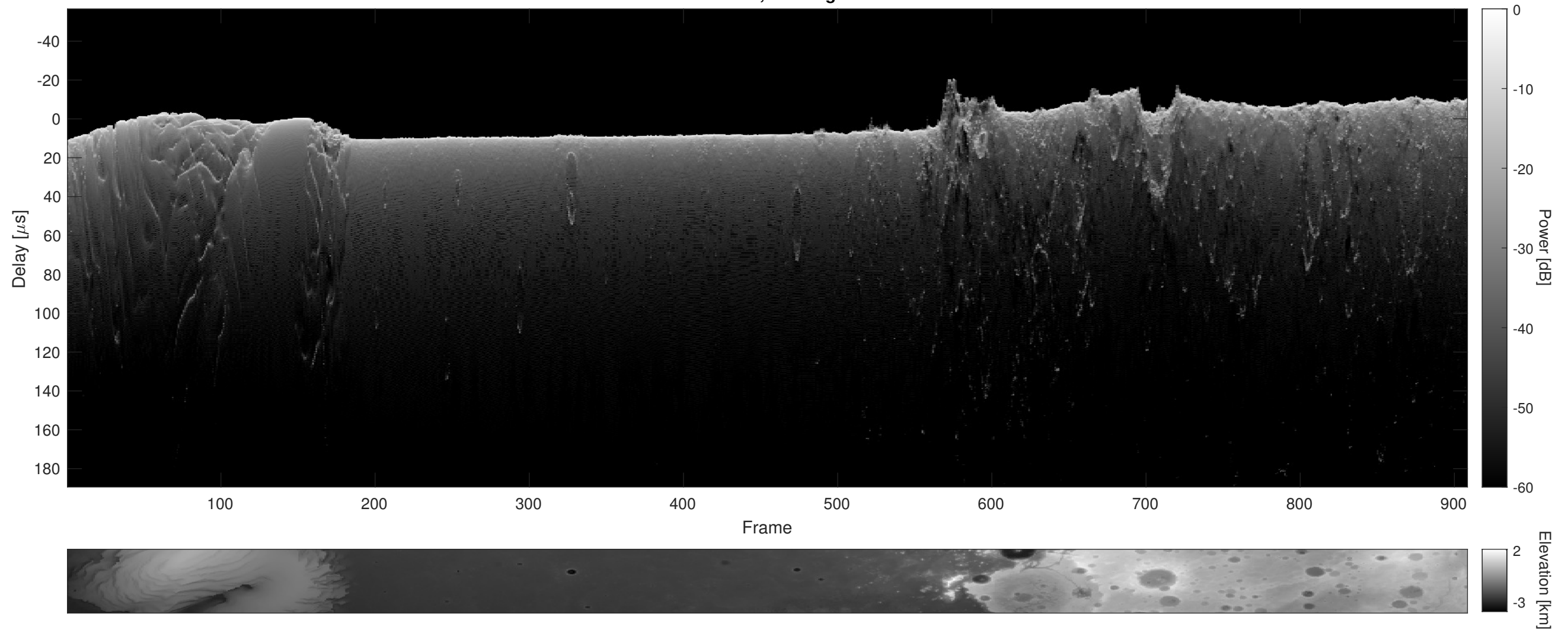
Orbit 11628, Cluttergram
