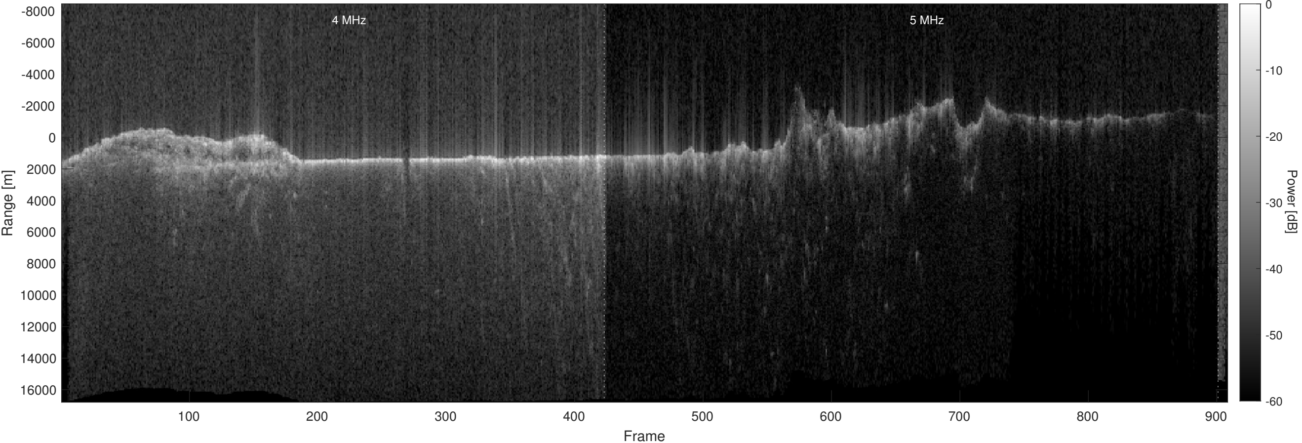
Orbit 11628, Optimized, No Window, Depth-Corrected, Channel 2
