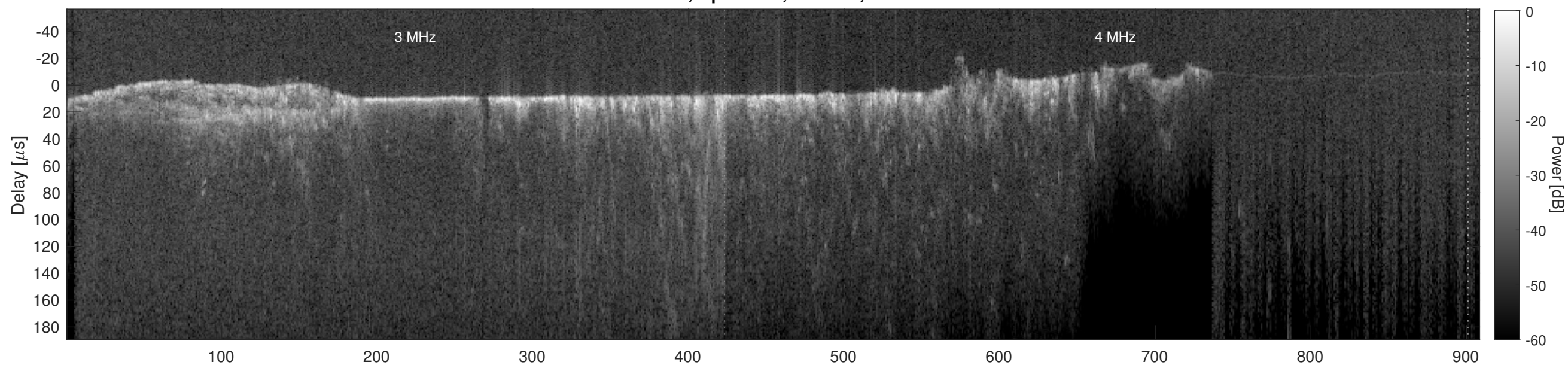
Orbit 11628, Cluttergram
