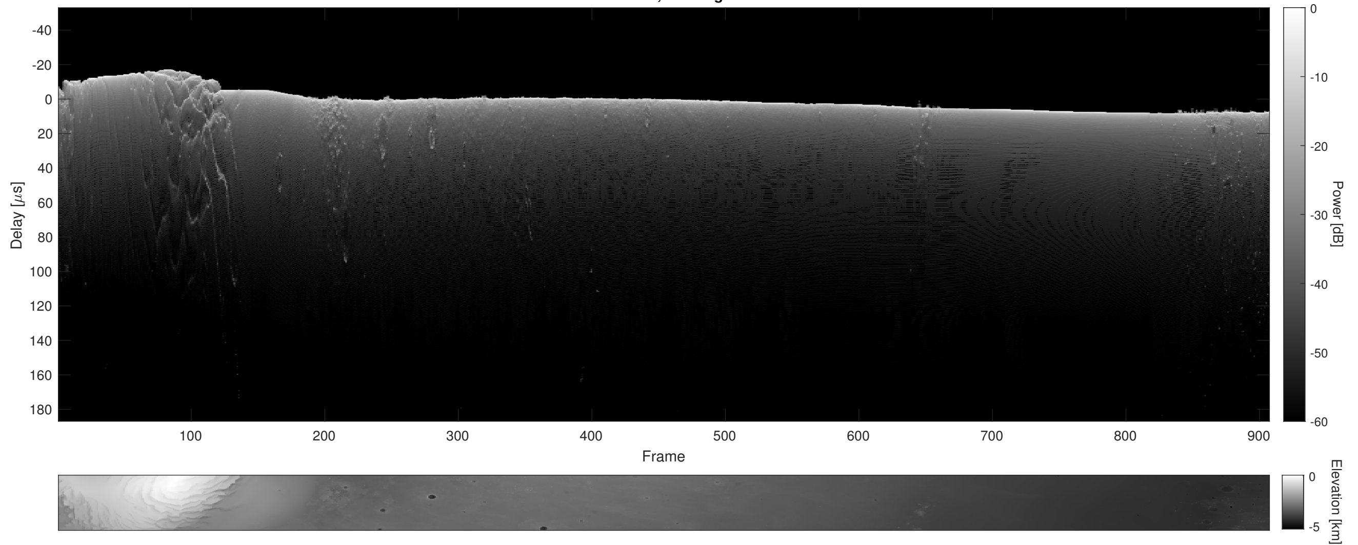
Orbit 11630, Cluttergram
