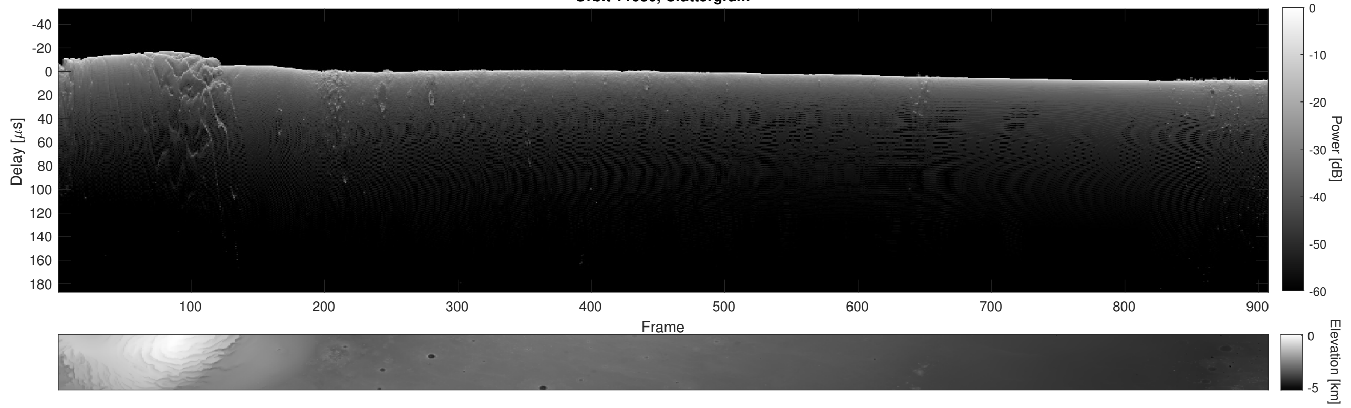
Orbit 11630, Cluttergram
