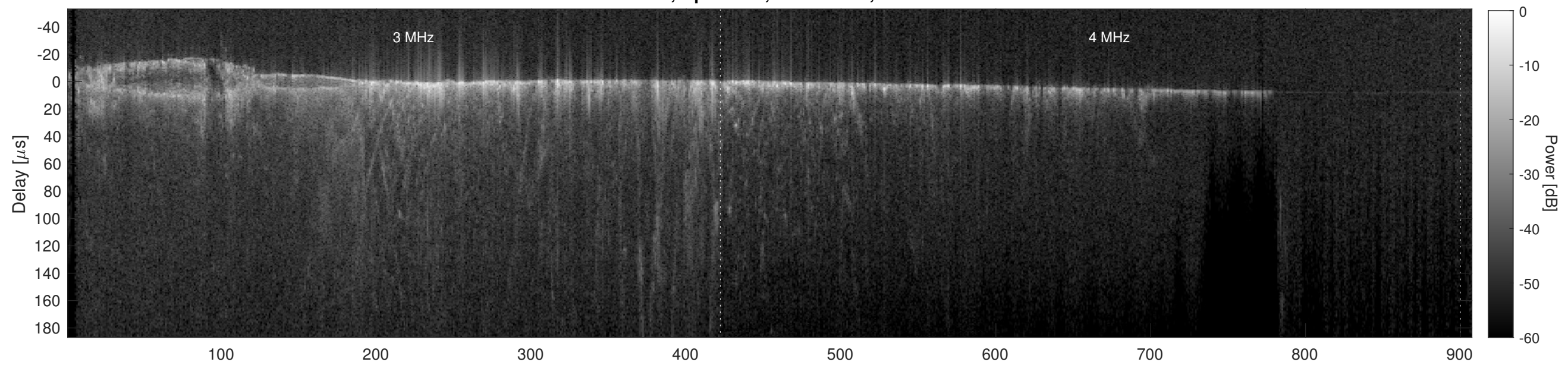
Orbit 11630, Cluttergram
