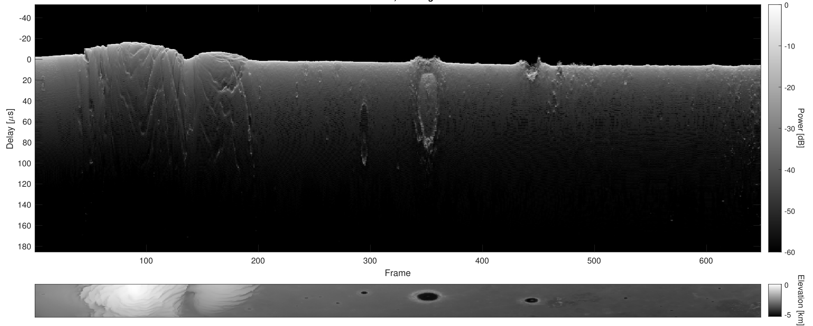
Orbit 11632, Cluttergram
