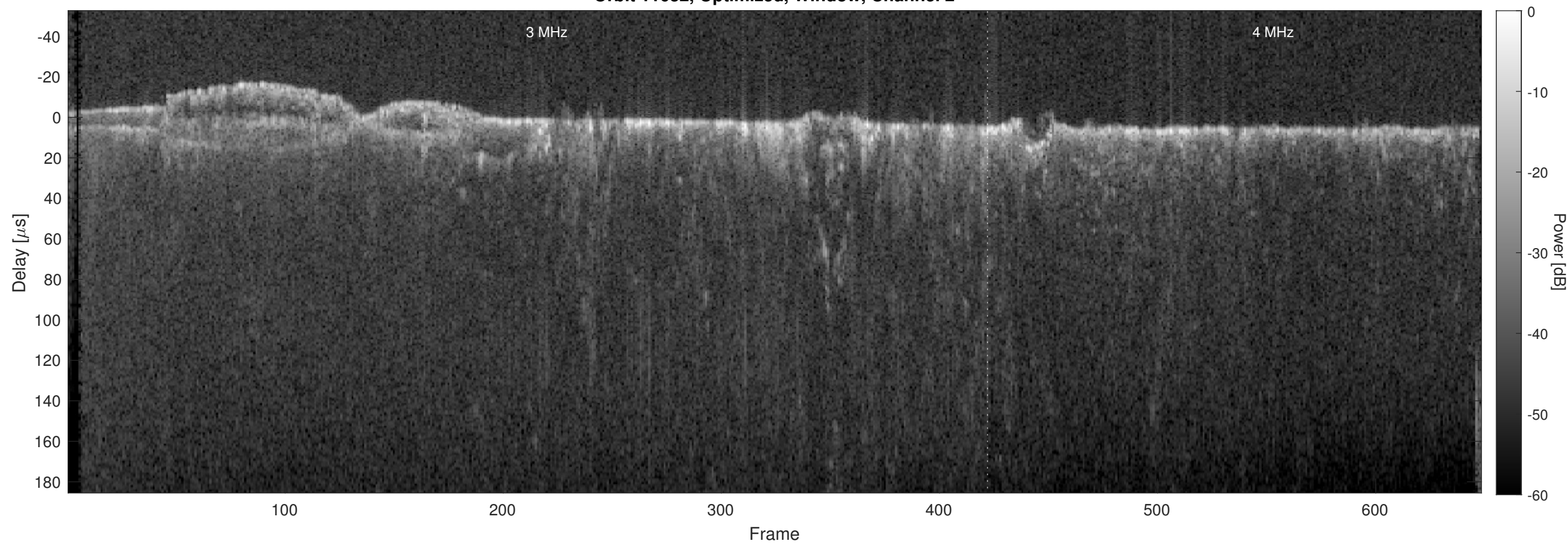
Orbit 11632, Optimized, Window, Channel 2
