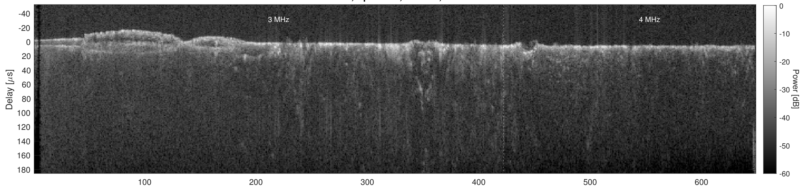
Orbit 11632, Cluttergram
