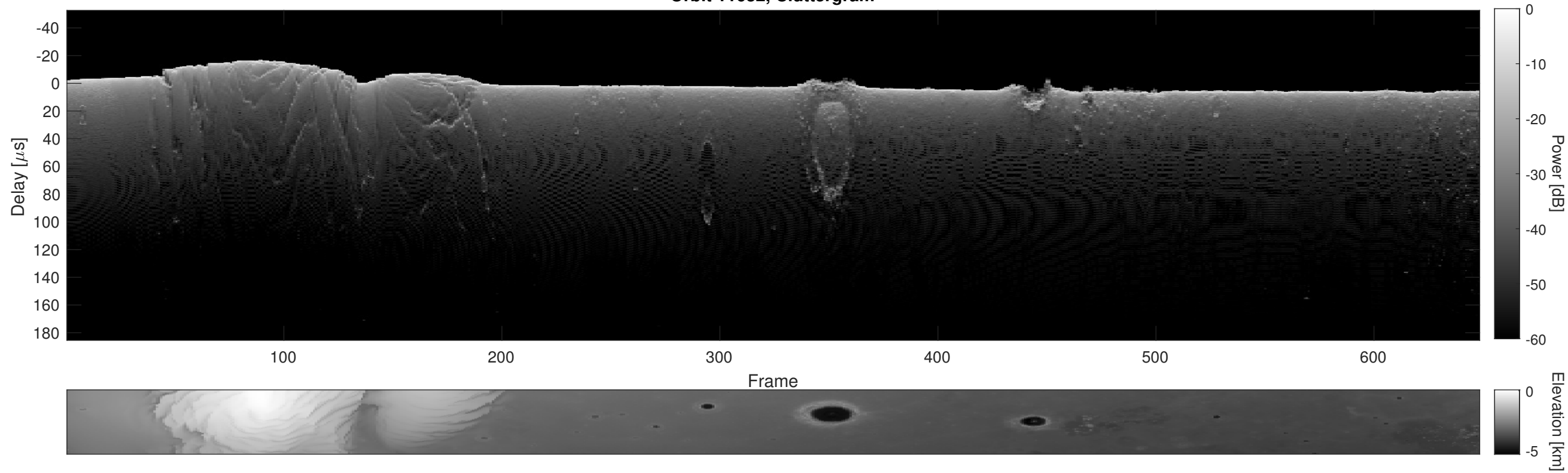
Orbit 11632, Cluttergram
