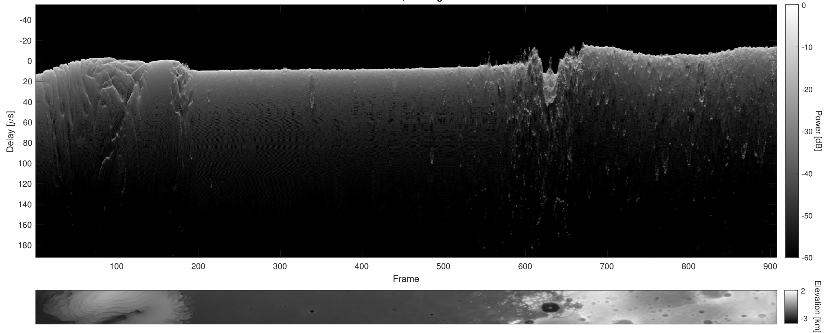
Orbit 11635, Cluttergram
