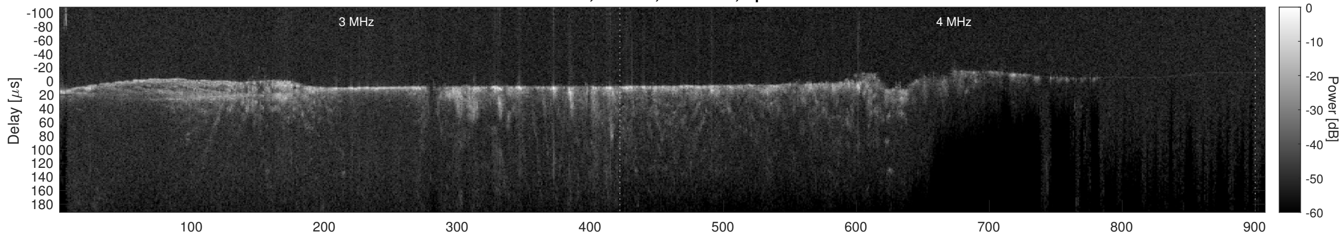
Orbit 11635, Cluttergram
