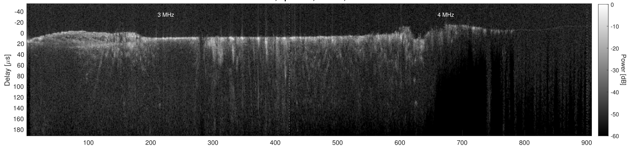
Orbit 11635, Cluttergram
