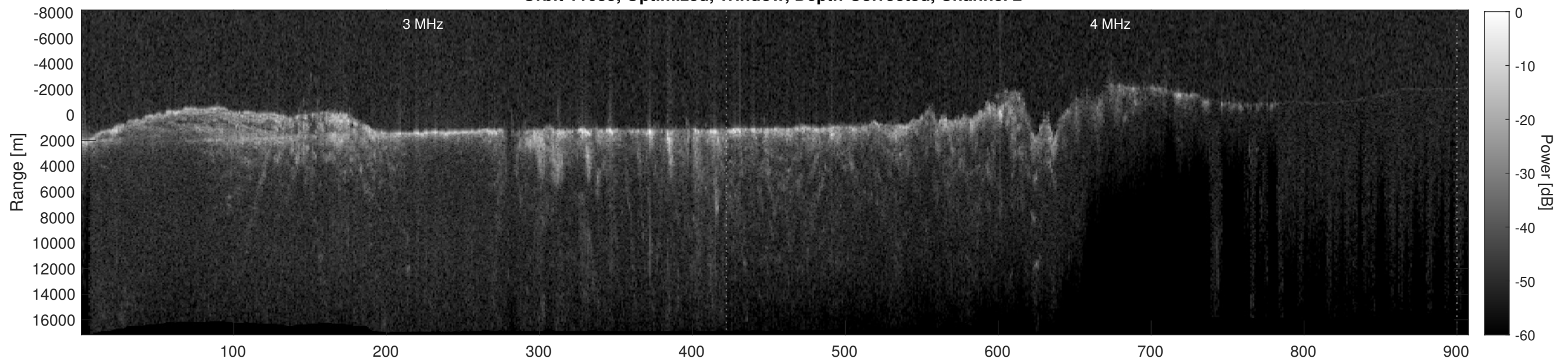
Orbit 11635, Depth-Corrected Cluttergram
