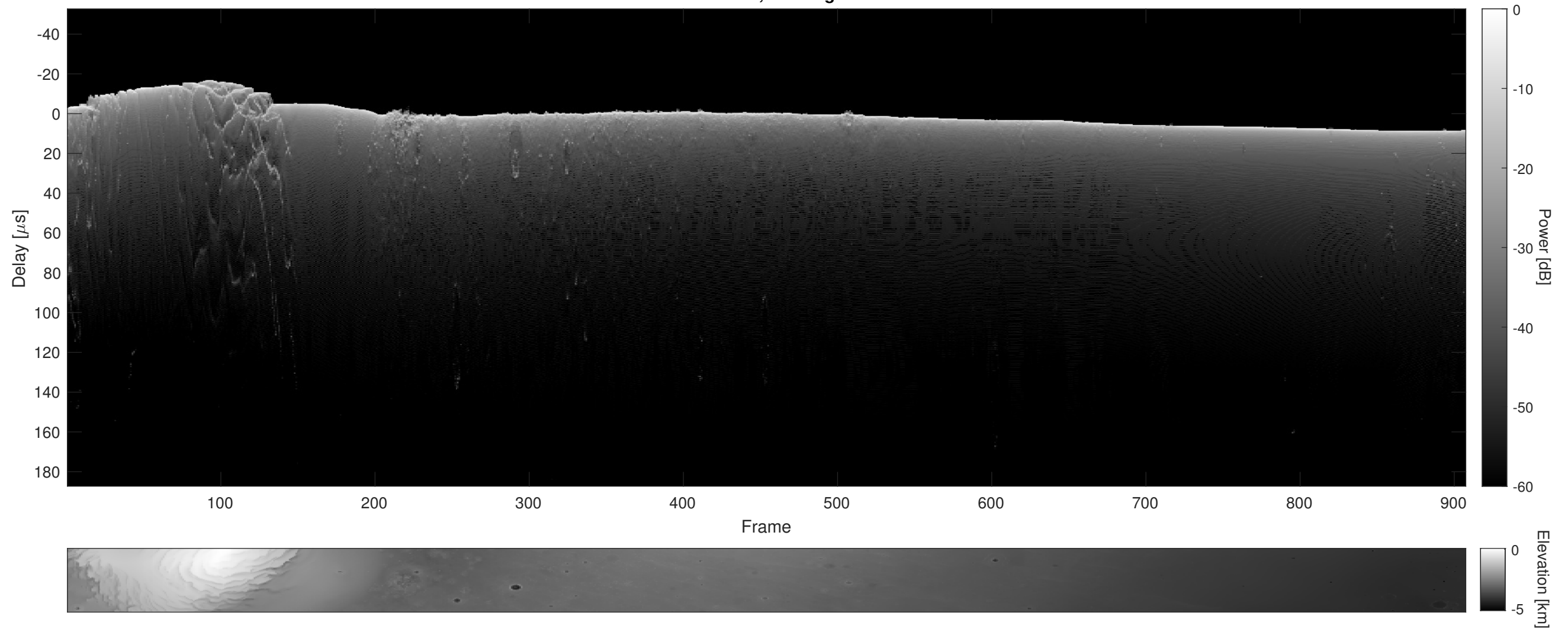
Orbit 11637, Cluttergram
