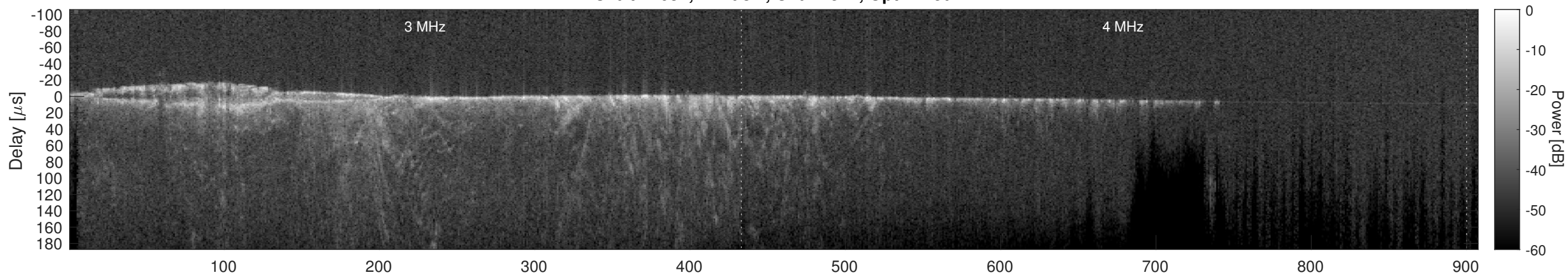
Orbit 11637, Cluttergram
