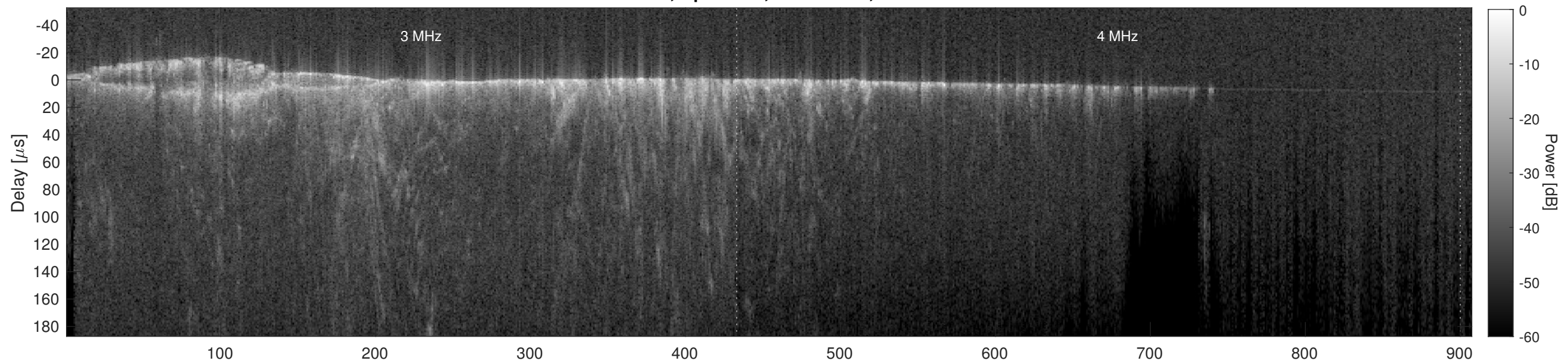
Orbit 11637, Cluttergram
