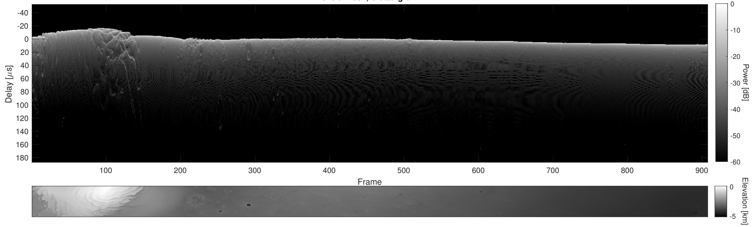
Orbit 11637, Cluttergram
