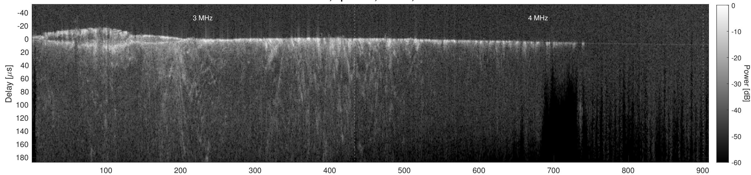
Orbit 11637, Cluttergram
