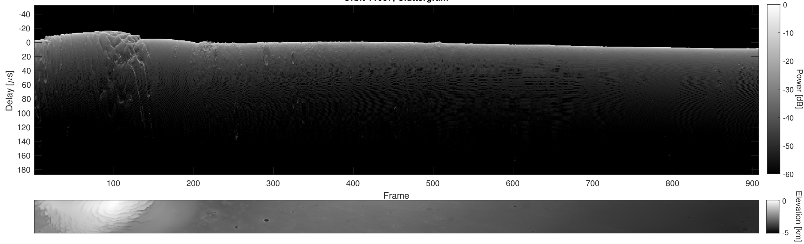
Orbit 11637, Cluttergram
