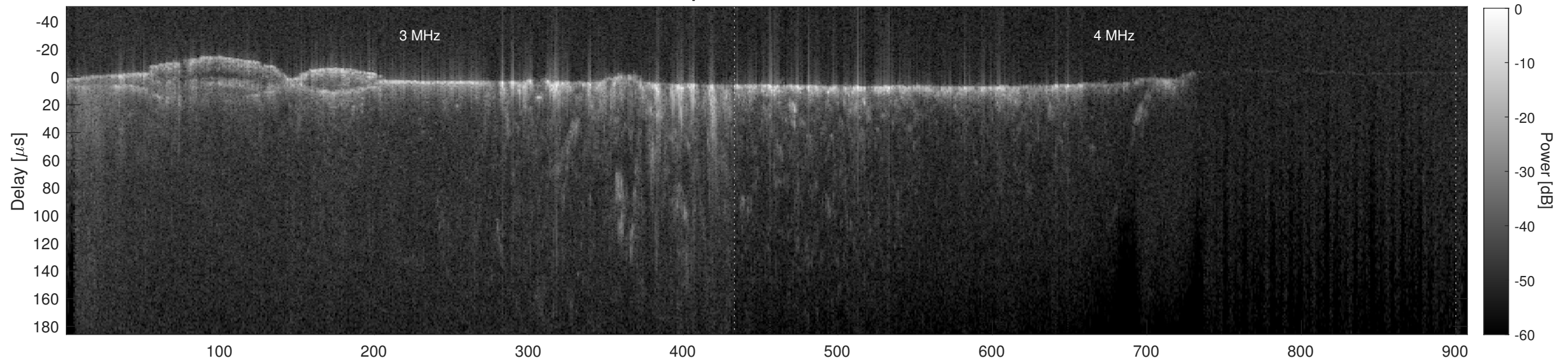
Orbit 11639, Cluttergram
