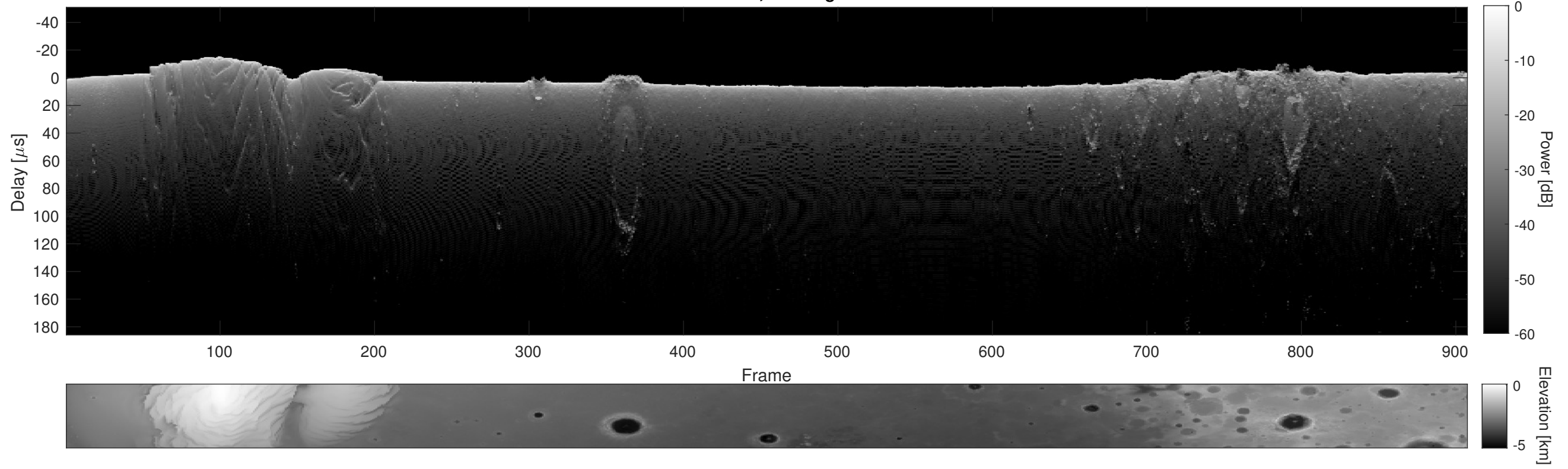
Orbit 11639, Cluttergram
