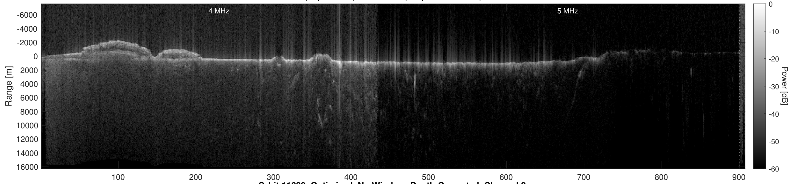
Orbit 11639, Optimized, No Window, Depth-Corrected, Channel 2
