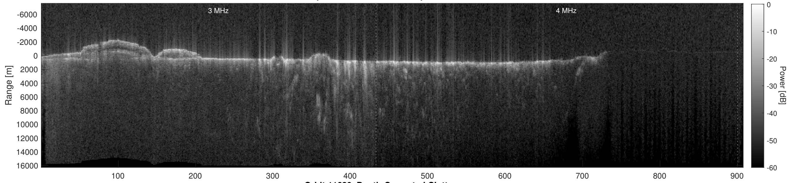
Orbit 11639, Depth-Corrected Cluttergram
