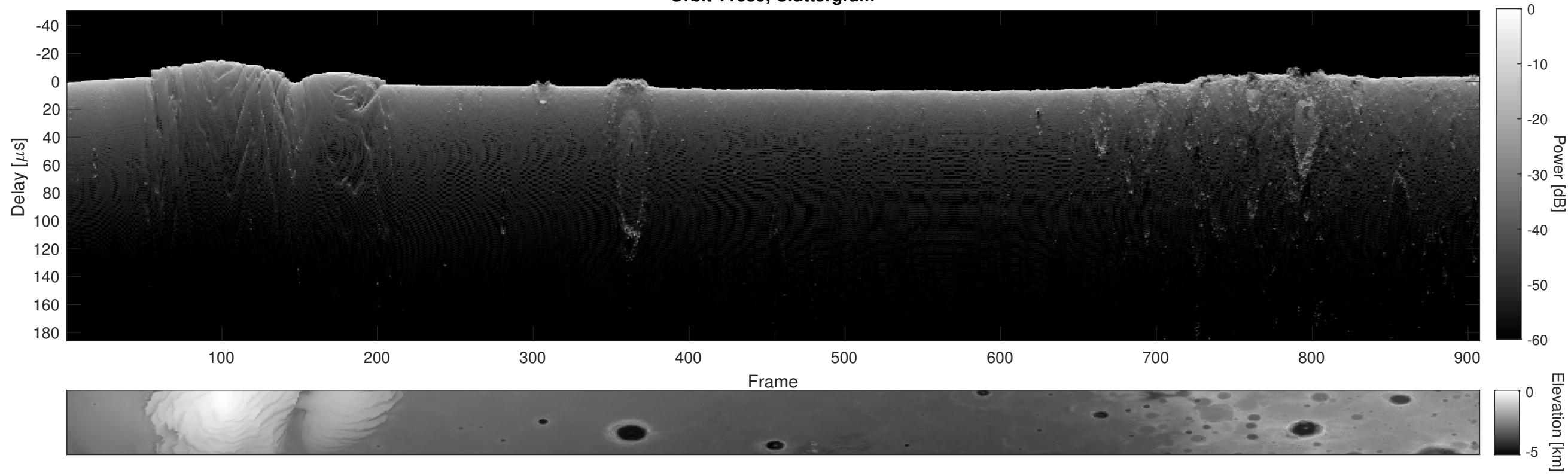
Orbit 11639, Cluttergram
