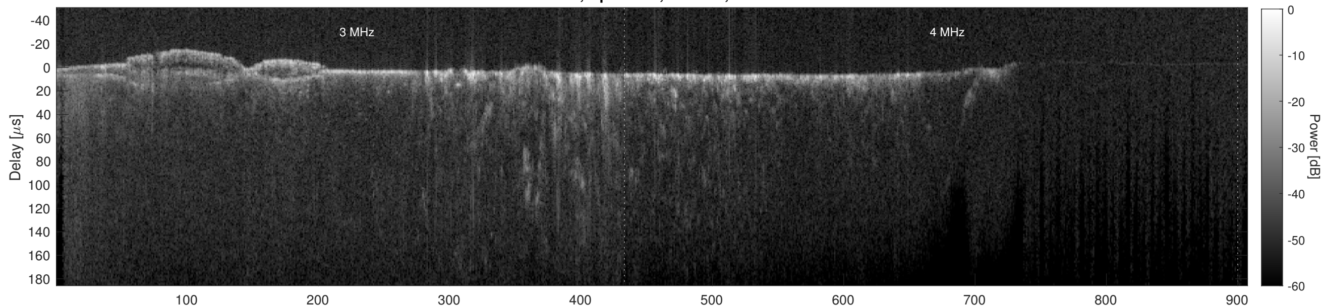
Orbit 11639, Cluttergram
