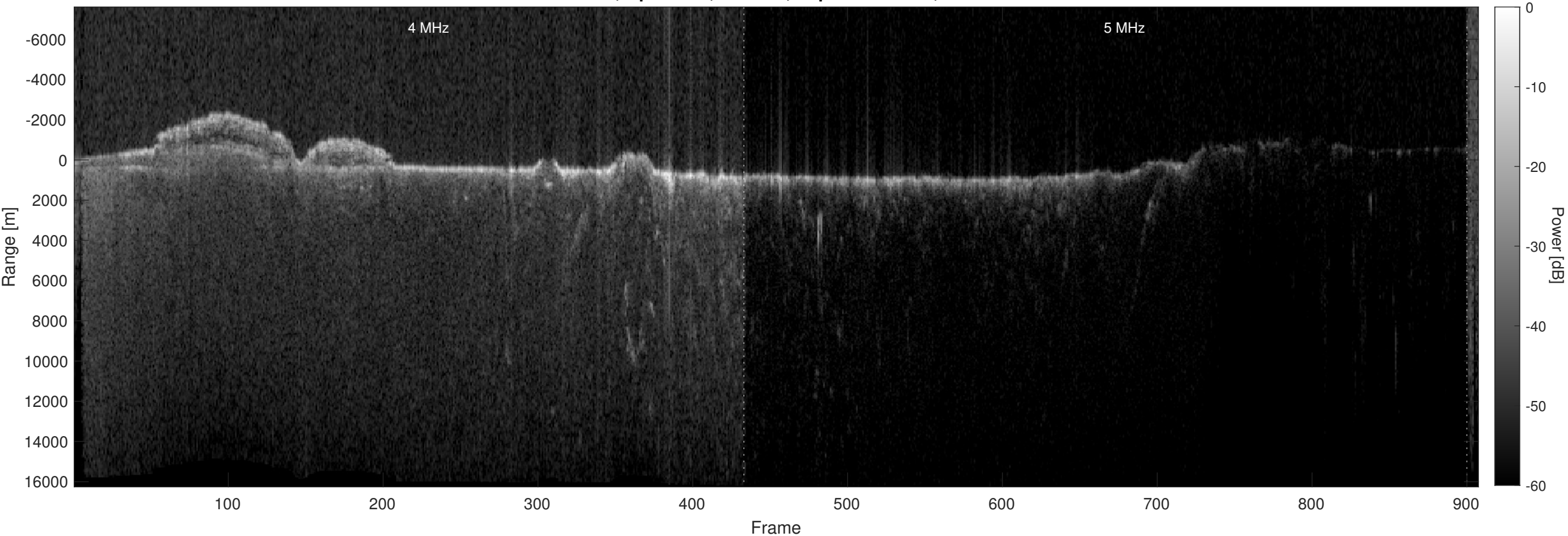
Orbit 11639, Optimized, Window, Depth-Corrected, Channel 2
