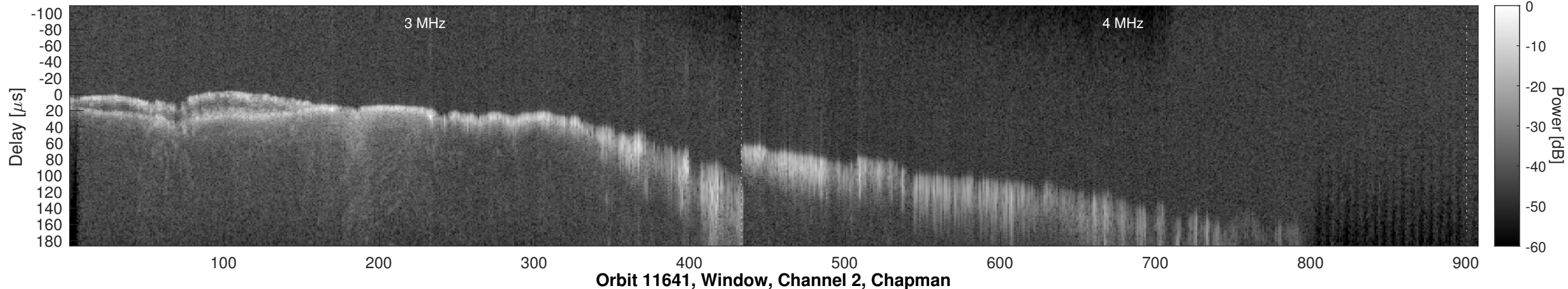
Orbit 11641, Window, Channel 2, Uncorrected
