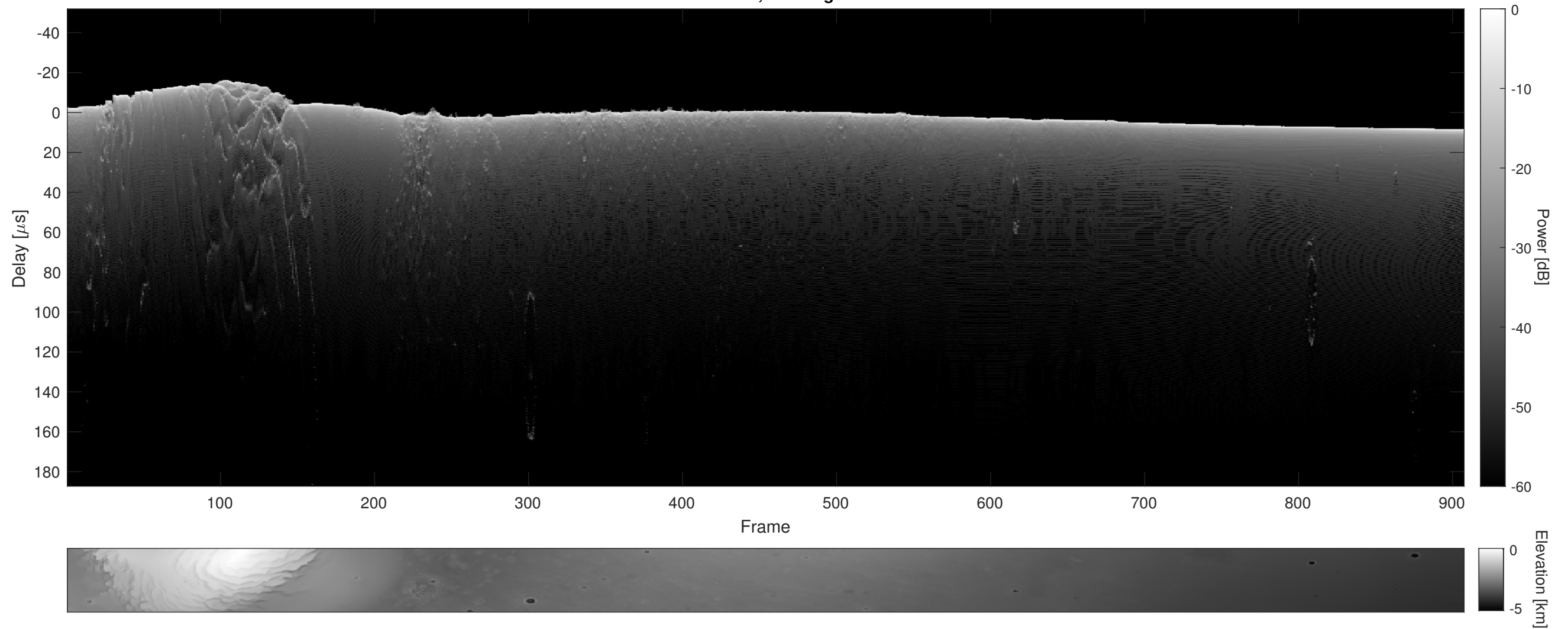
Orbit 11644, Cluttergram
