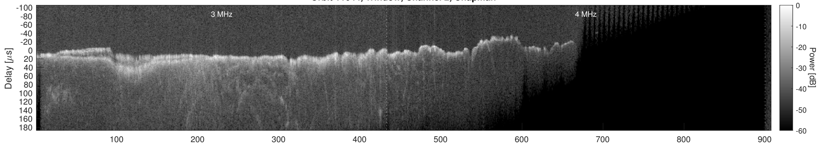
Orbit 11644, Window, Channel 2, Optimized
