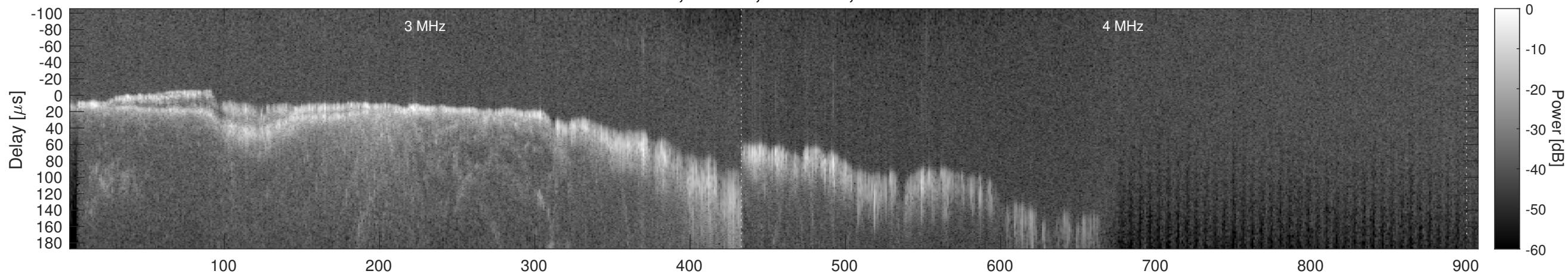
Orbit 11644, Window, Channel 2, Chapman
