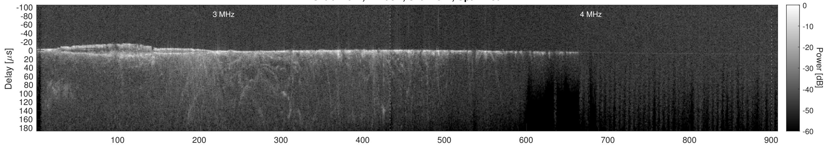
Orbit 11644, Cluttergram
