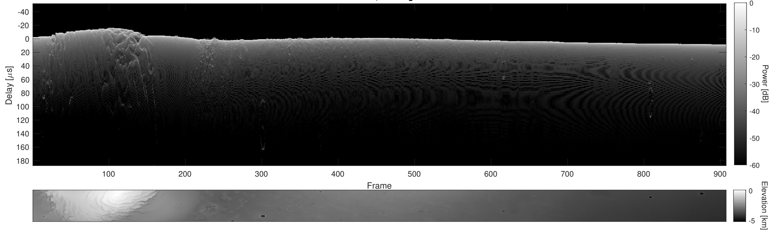
Orbit 11644, Cluttergram
