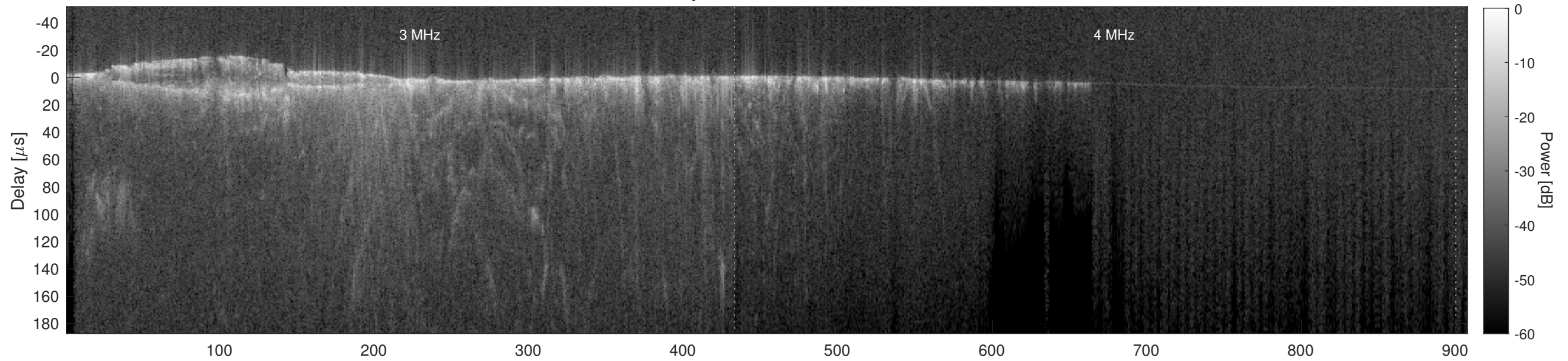
Orbit 11644, Cluttergram
