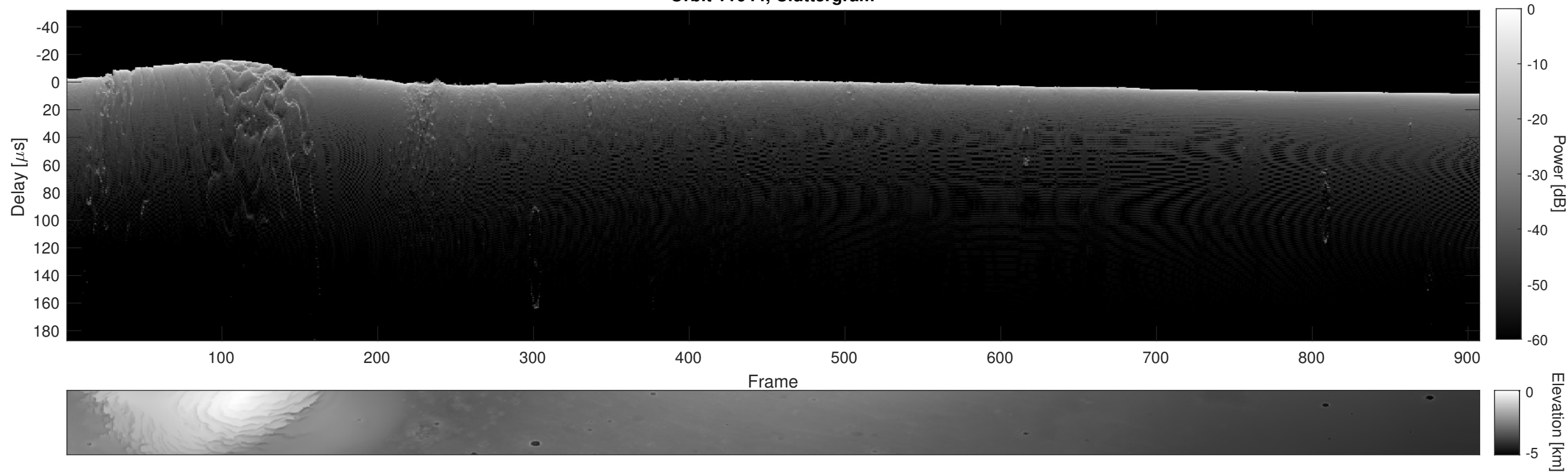
Orbit 11644, Cluttergram
