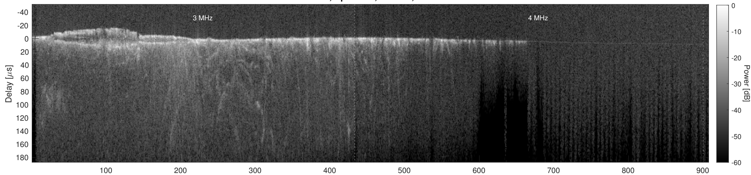
Orbit 11644, Cluttergram
