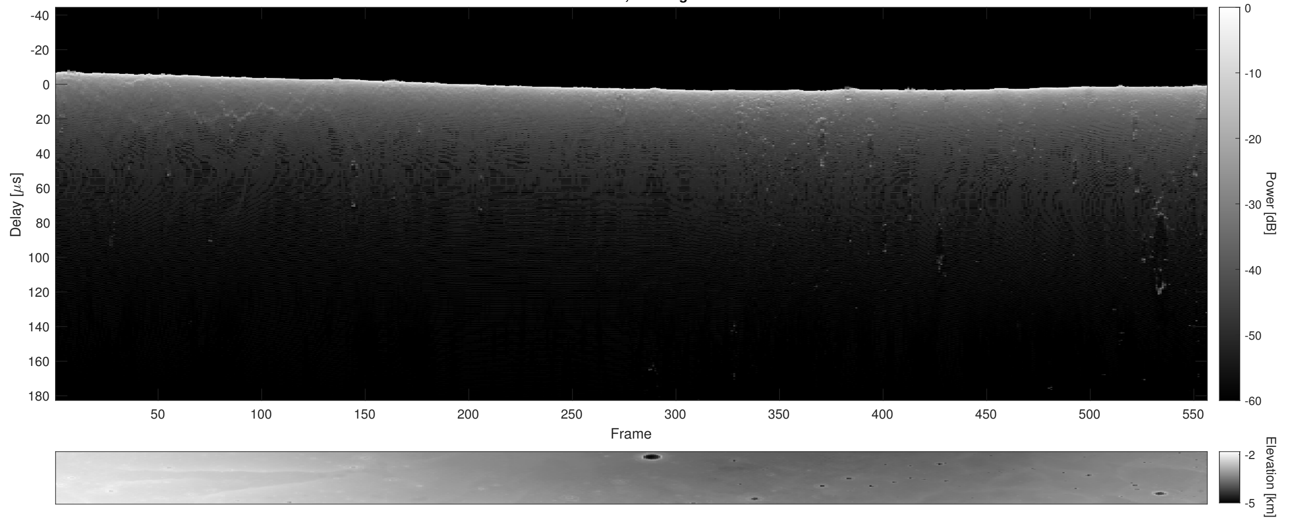
Orbit 11645, Cluttergram
