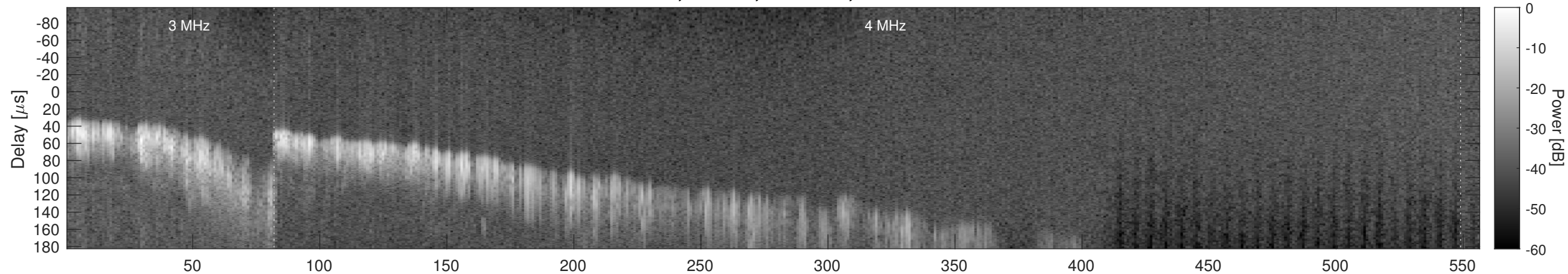
Orbit 11645, Window, Channel 2, Chapman
