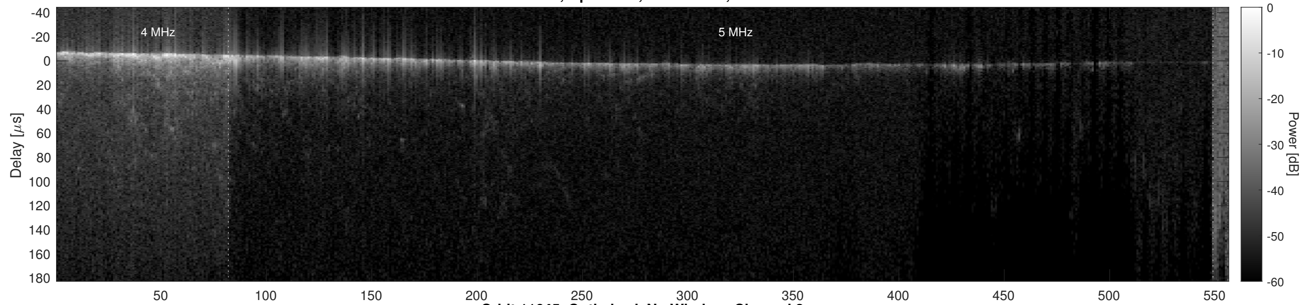
Orbit 11645, Optimized, No Window, Channel 2
