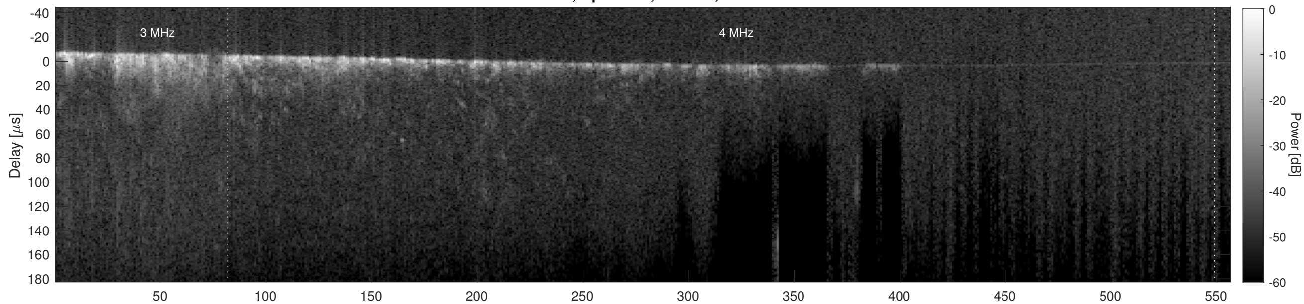
Orbit 11645, Cluttergram
