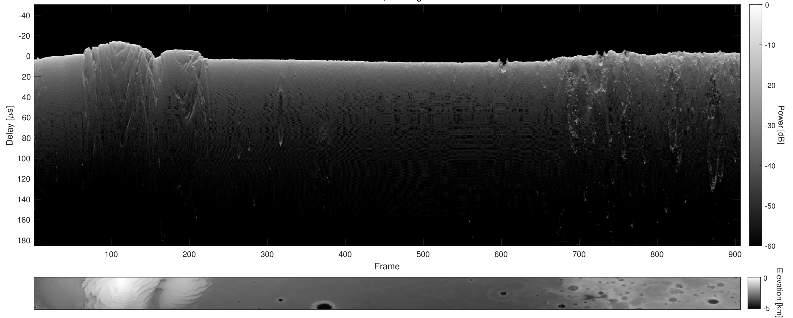
Orbit 11646, Cluttergram
