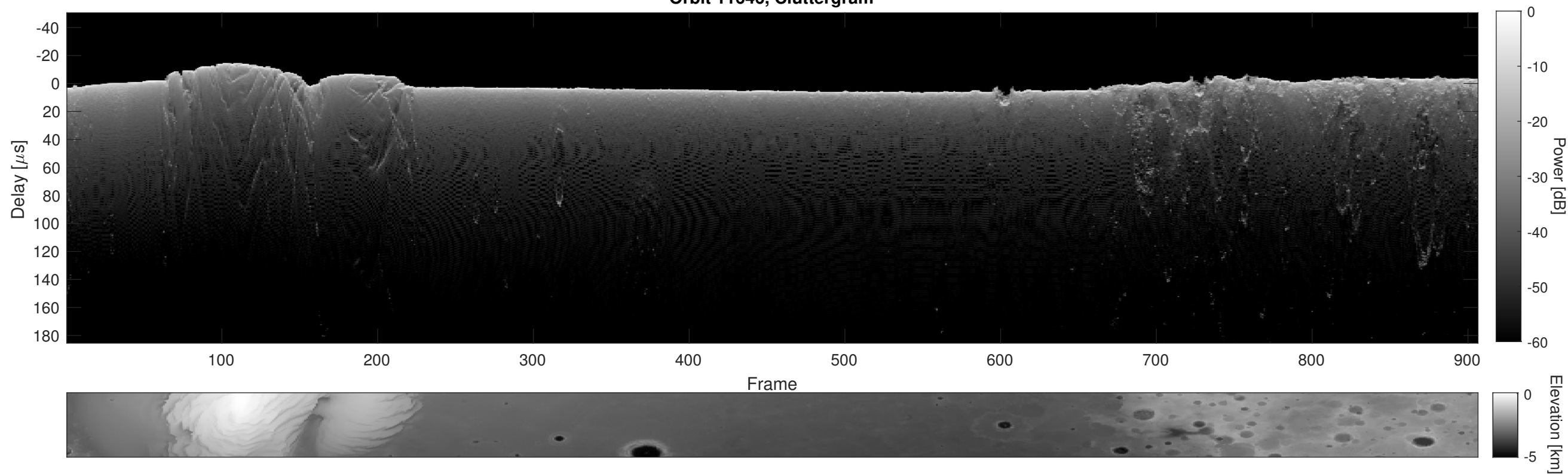
Orbit 11646, Cluttergram
