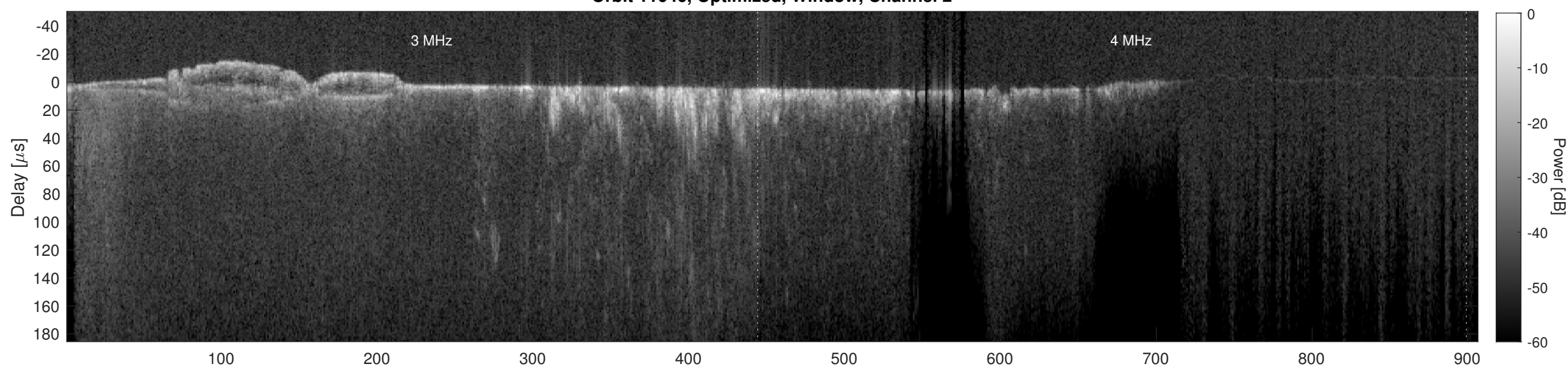
Orbit 11646, Cluttergram
