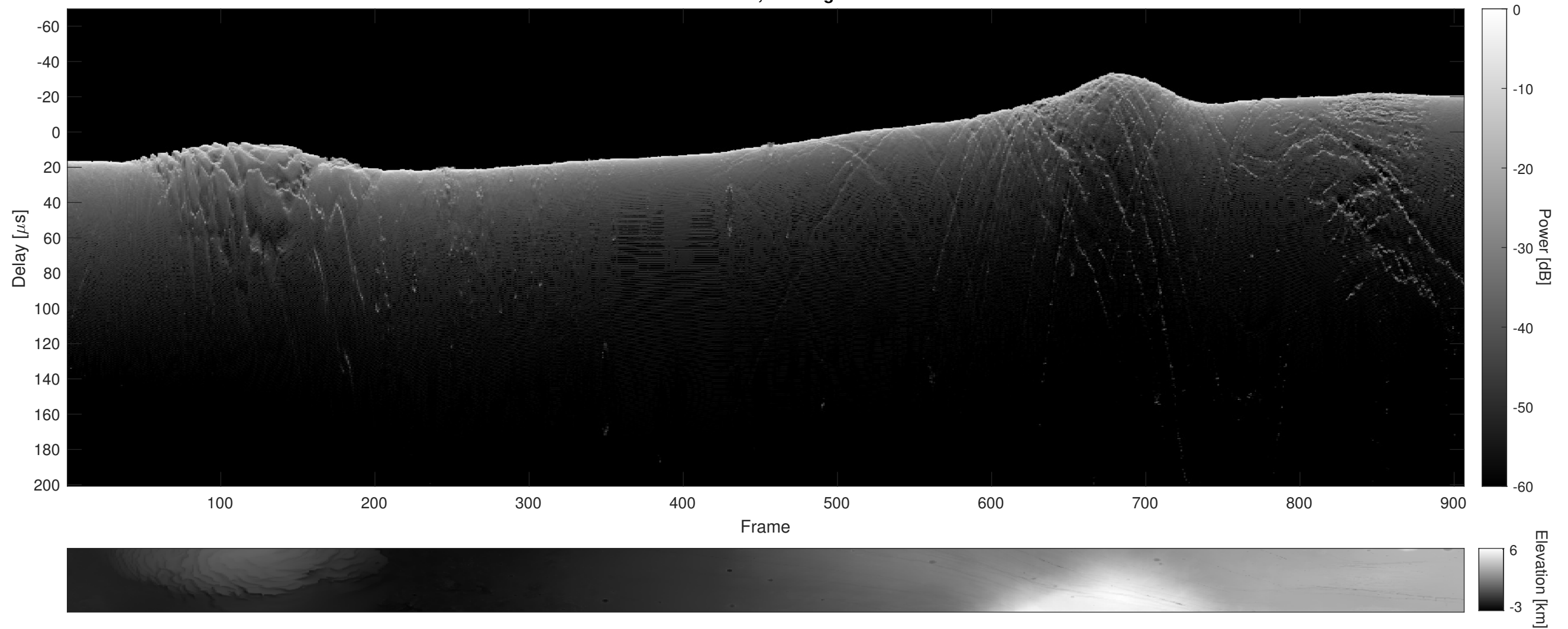
Orbit 11647, Cluttergram
