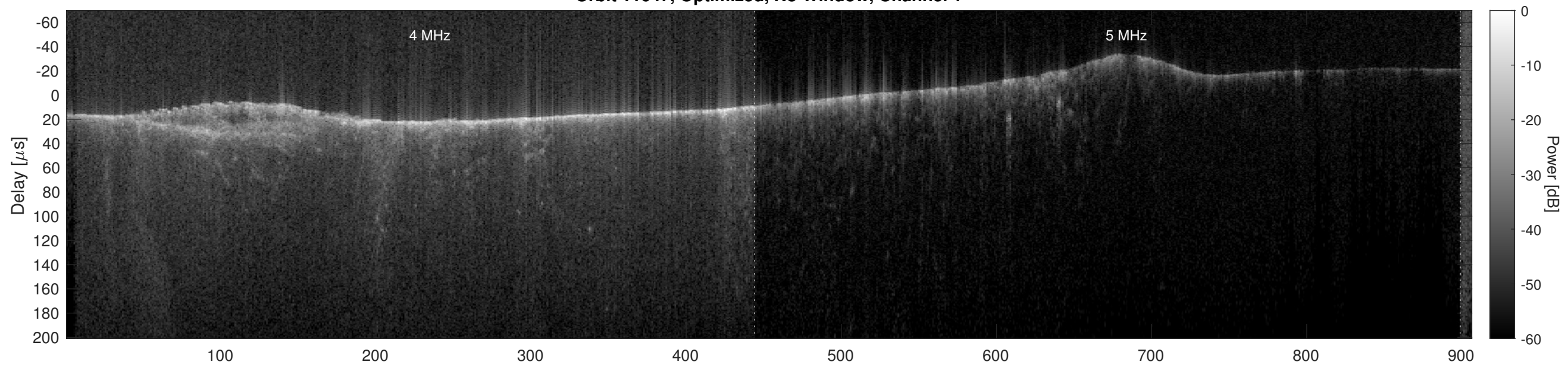
Orbit 11647, Optimized, No Window, Channel 2
