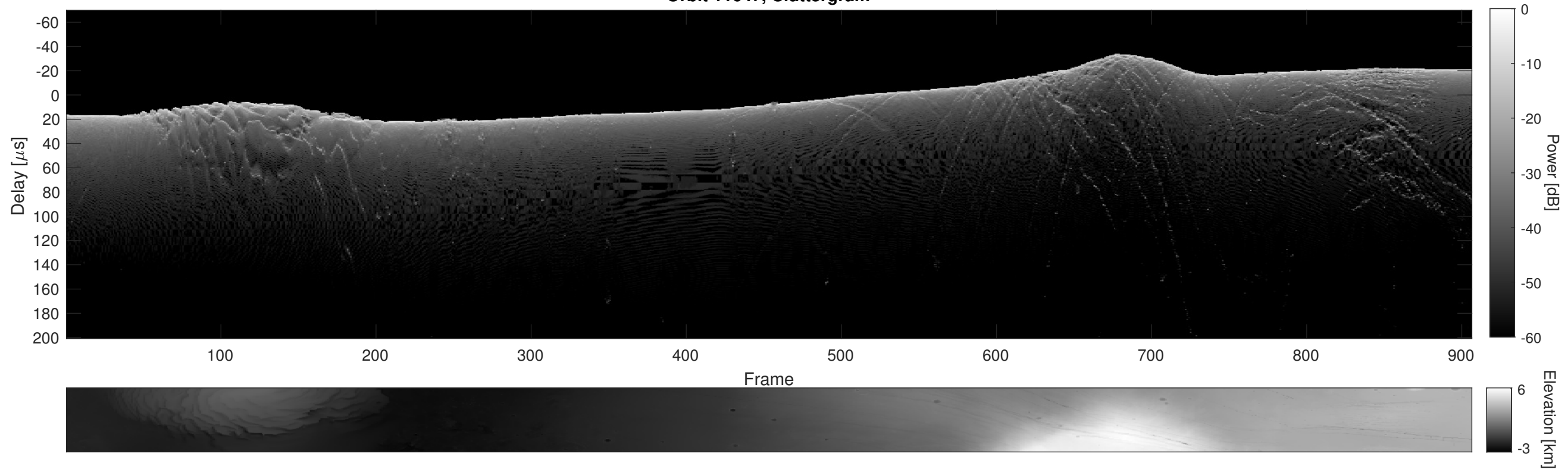
Orbit 11647, Cluttergram
