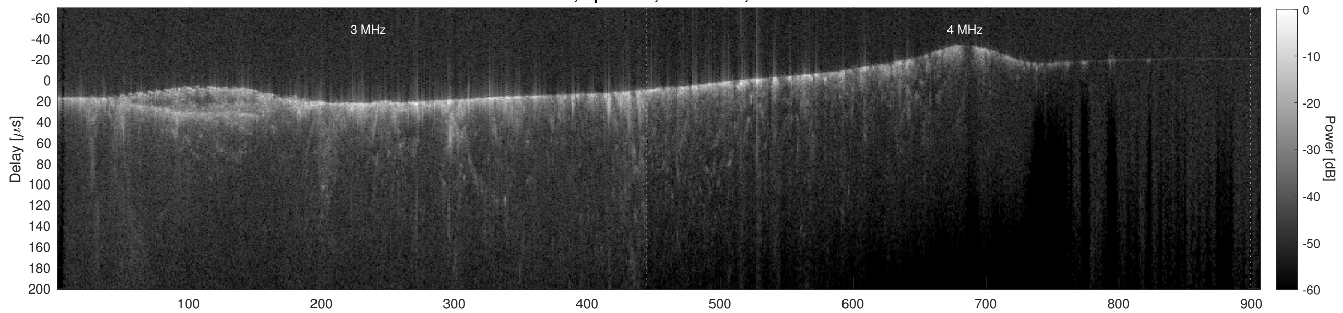
Orbit 11647, Cluttergram
