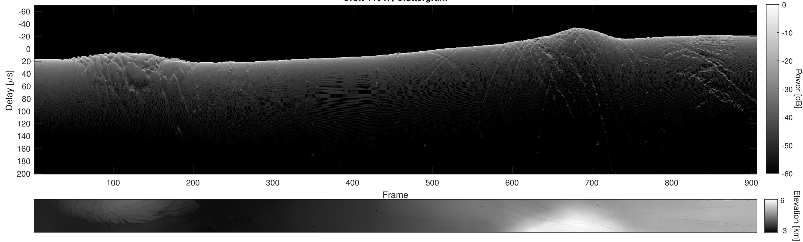
Orbit 11647, Cluttergram
