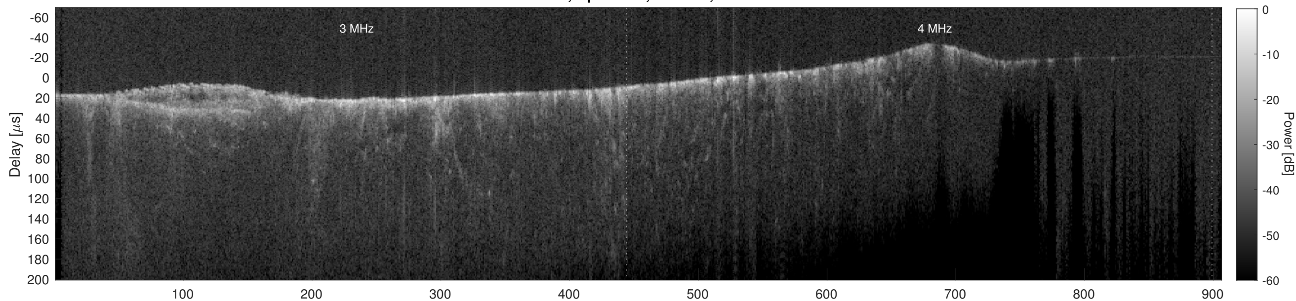
Orbit 11647, Cluttergram
