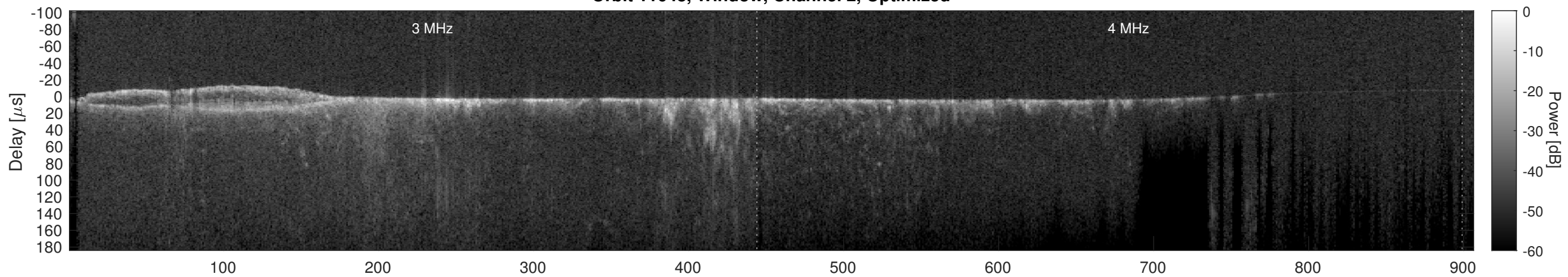
Orbit 11648, Cluttergram
