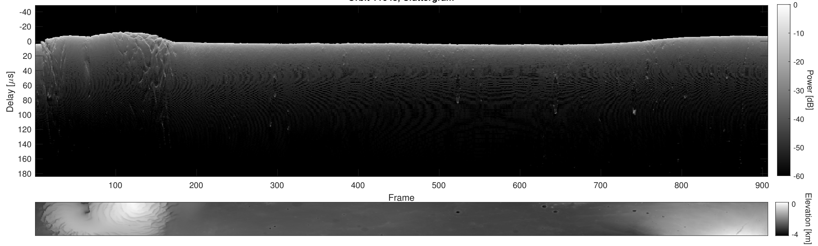
Orbit 11648, Cluttergram
