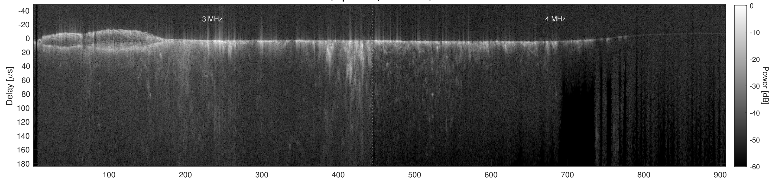
Orbit 11648, Cluttergram
