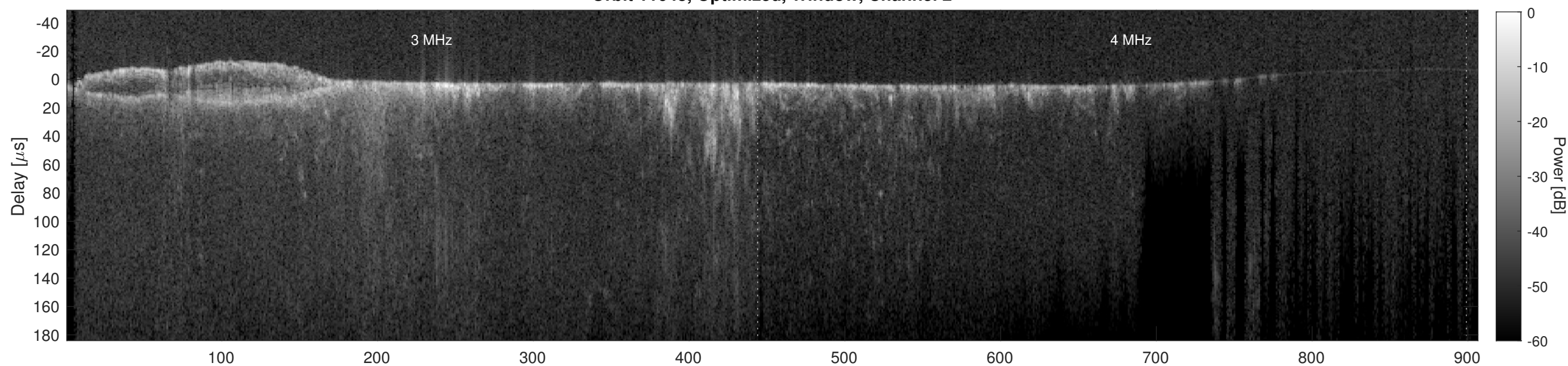
Orbit 11648, Cluttergram
