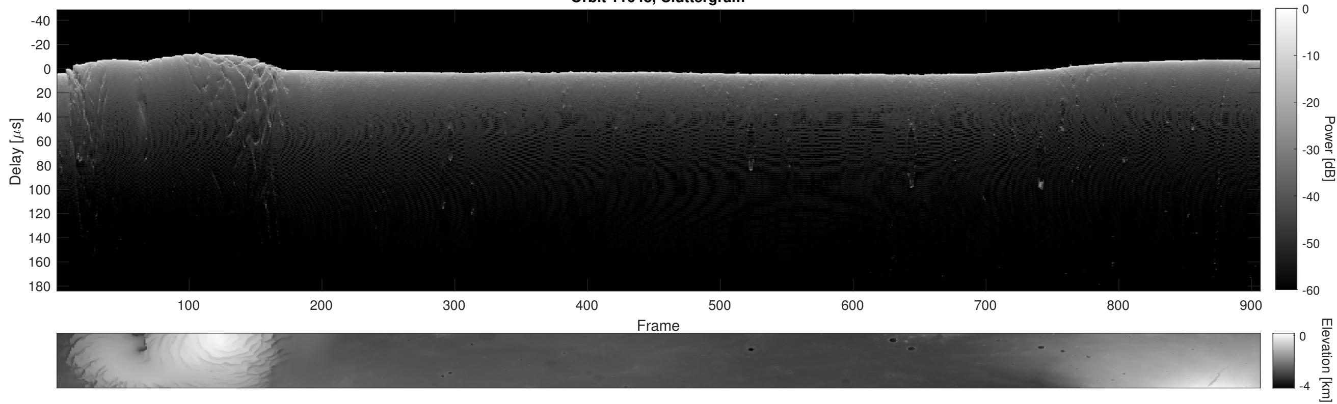
Orbit 11648, Cluttergram
