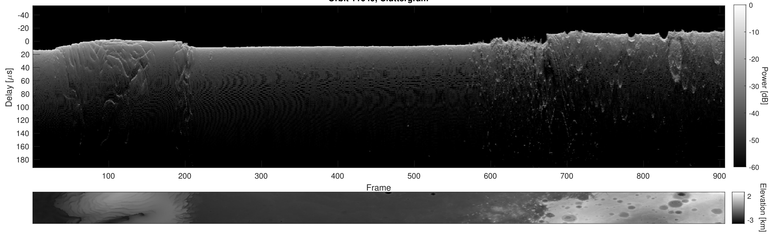
Orbit 11649, Cluttergram
