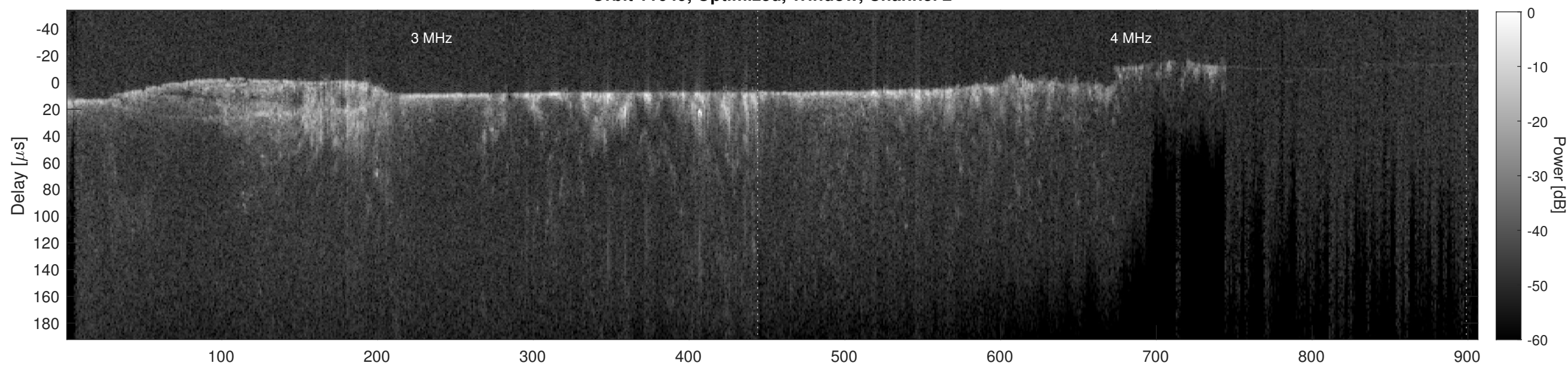
Orbit 11649, Cluttergram
