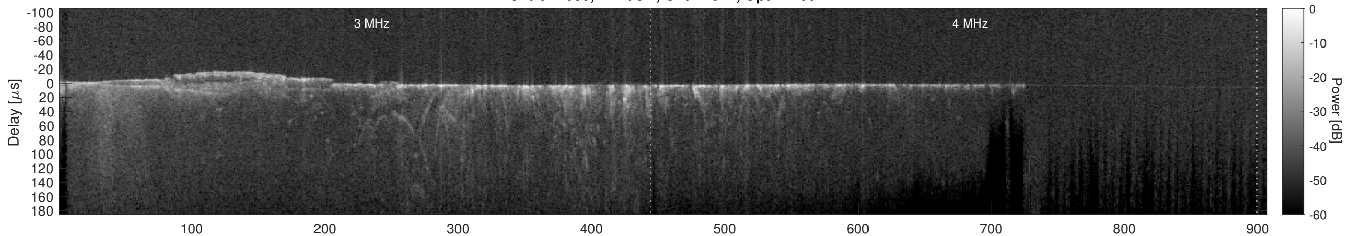
Orbit 11650, Cluttergram
