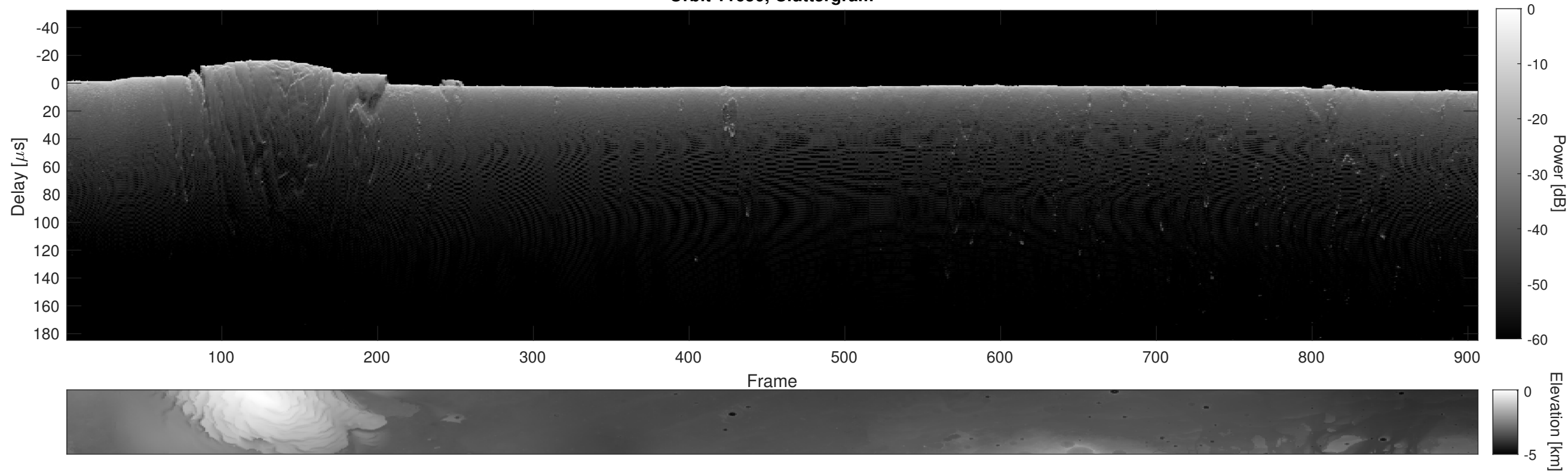
Orbit 11650, Cluttergram
