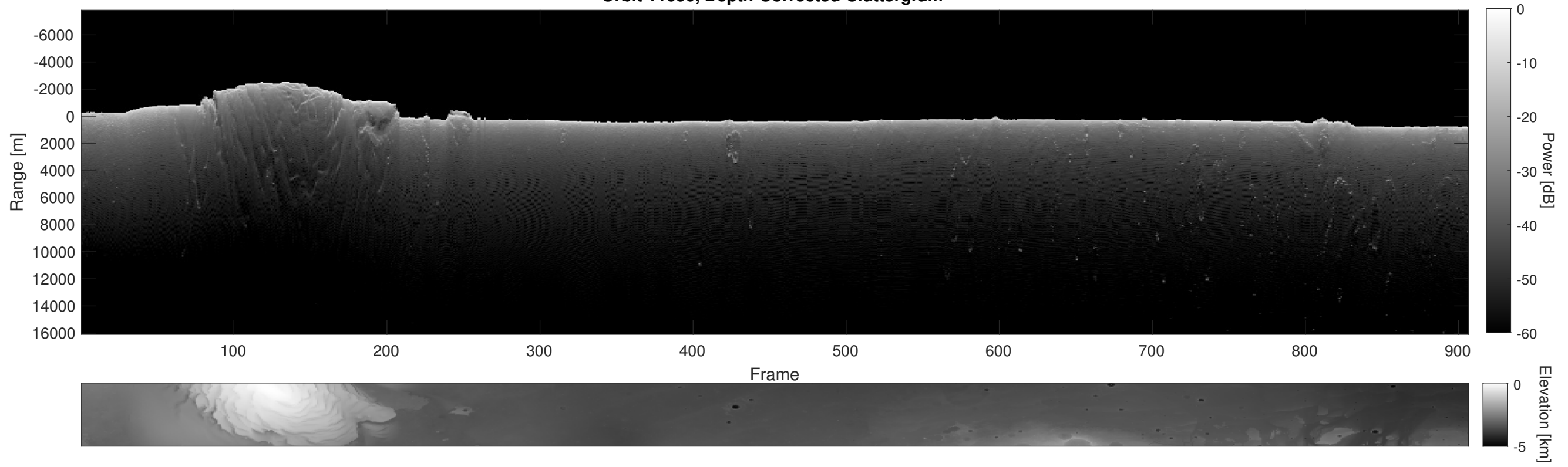
Orbit 11650, Depth-Corrected Cluttergram
