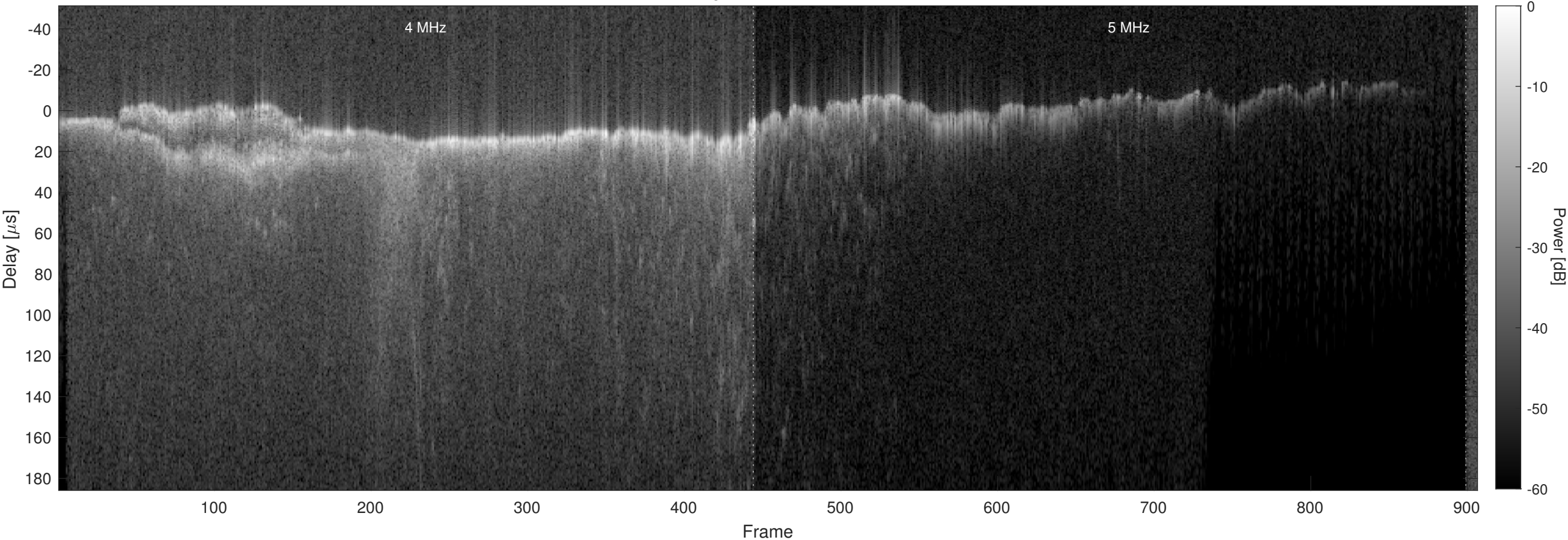
Orbit 11651, Chapman, No Window, Channel 2
