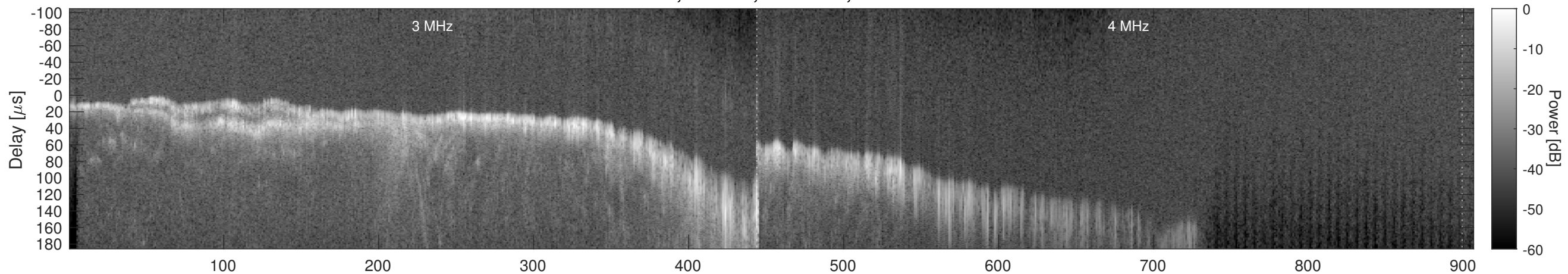
Orbit 11651, Window, Channel 2, Chapman
