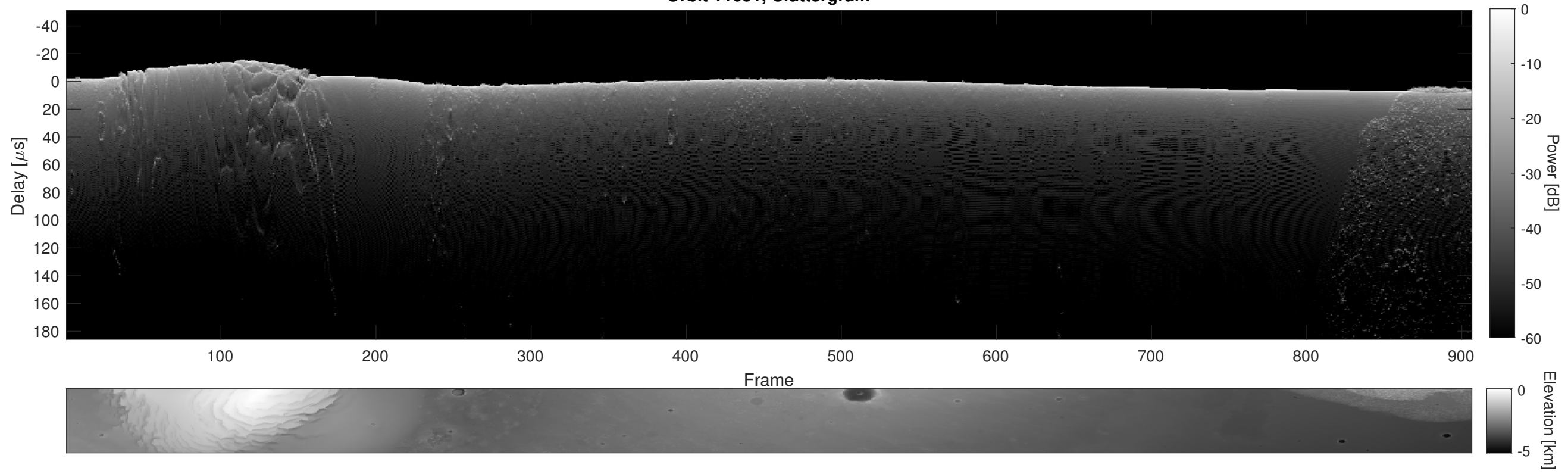
Orbit 11651, Cluttergram
